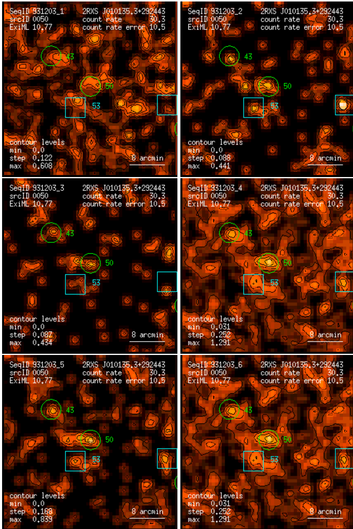
Figure 50: RASS 931203: detection 0050: band rate images, Gaussian filter: (1) PSPC channels 11 – 41, (2) 52 – 90, (3) 91 – 201, (4) 11 – 235, (5) 52 – 201, (6) 11 – 201. Broad band rates in counts/ks. Band rate contour levels in counts/ks/arcmin 2 .
