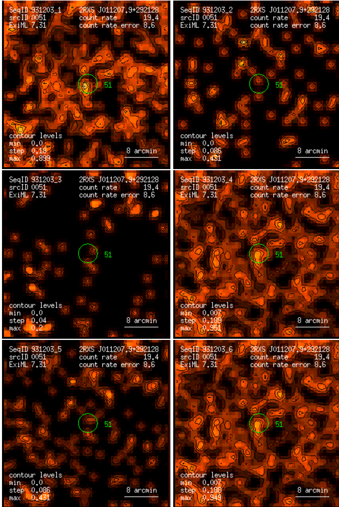
Figure 51: RASS 931203: detection 0051: band rate images, Gaussian filter: (1) PSPC channels 11 – 41, (2) 52 – 90, (3) 91 – 201, (4) 11 – 235, (5) 52 – 201, (6) 11 – 201. Broad band rates in counts/ks. Band rate contour levels in counts/ks/arcmin 2 .
