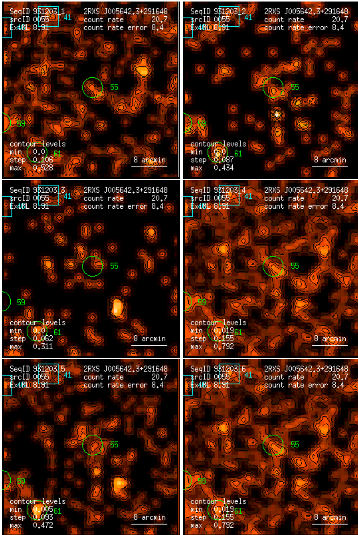
Figure 55: RASS 931203: detection 0055: band rate images, Gaussian filter: (1) PSPC channels 11 – 41, (2) 52 – 90, (3) 91 – 201, (4) 11 – 235, (5) 52 – 201, (6) 11 – 201. Broad band rates in counts/ks. Band rate contour levels in counts/ks/arcmin 2 .
