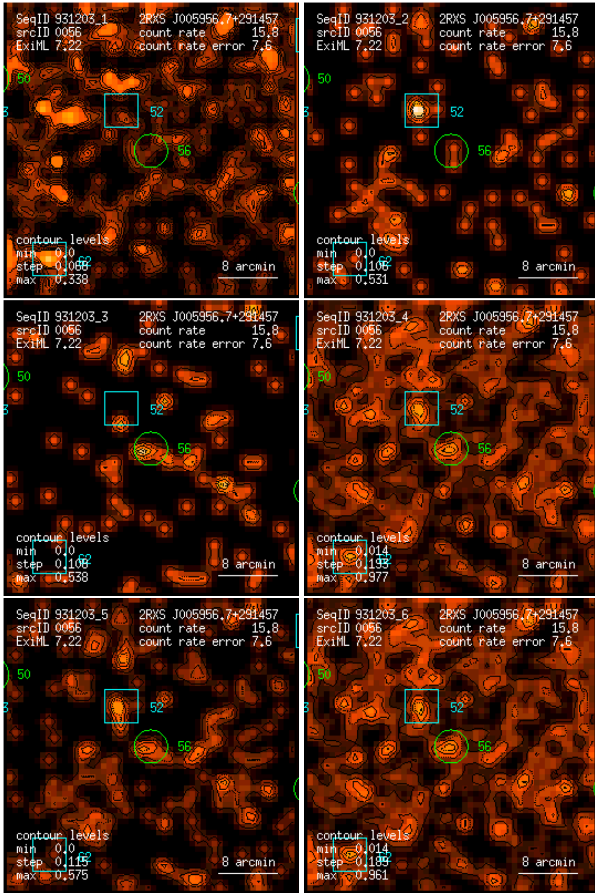
Figure 56: RASS 931203: detection 0056: band rate images, Gaussian filter: (1) PSPC channels 11 – 41, (2) 52 – 90, (3) 91 – 201, (4) 11 – 235, (5) 52 – 201, (6) 11 – 201. Broad band rates in counts/ks. Band rate contour levels in counts/ks/arcmin 2 .
