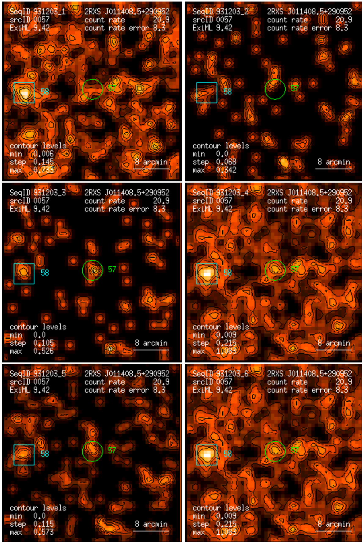
Figure 57: RASS 931203: detection 0057: band rate images, Gaussian filter: (1) PSPC channels 11 – 41, (2) 52 – 90, (3) 91 – 201, (4) 11 – 235, (5) 52 – 201, (6) 11 – 201. Broad band rates in counts/ks. Band rate contour levels in counts/ks/arcmin 2 .
