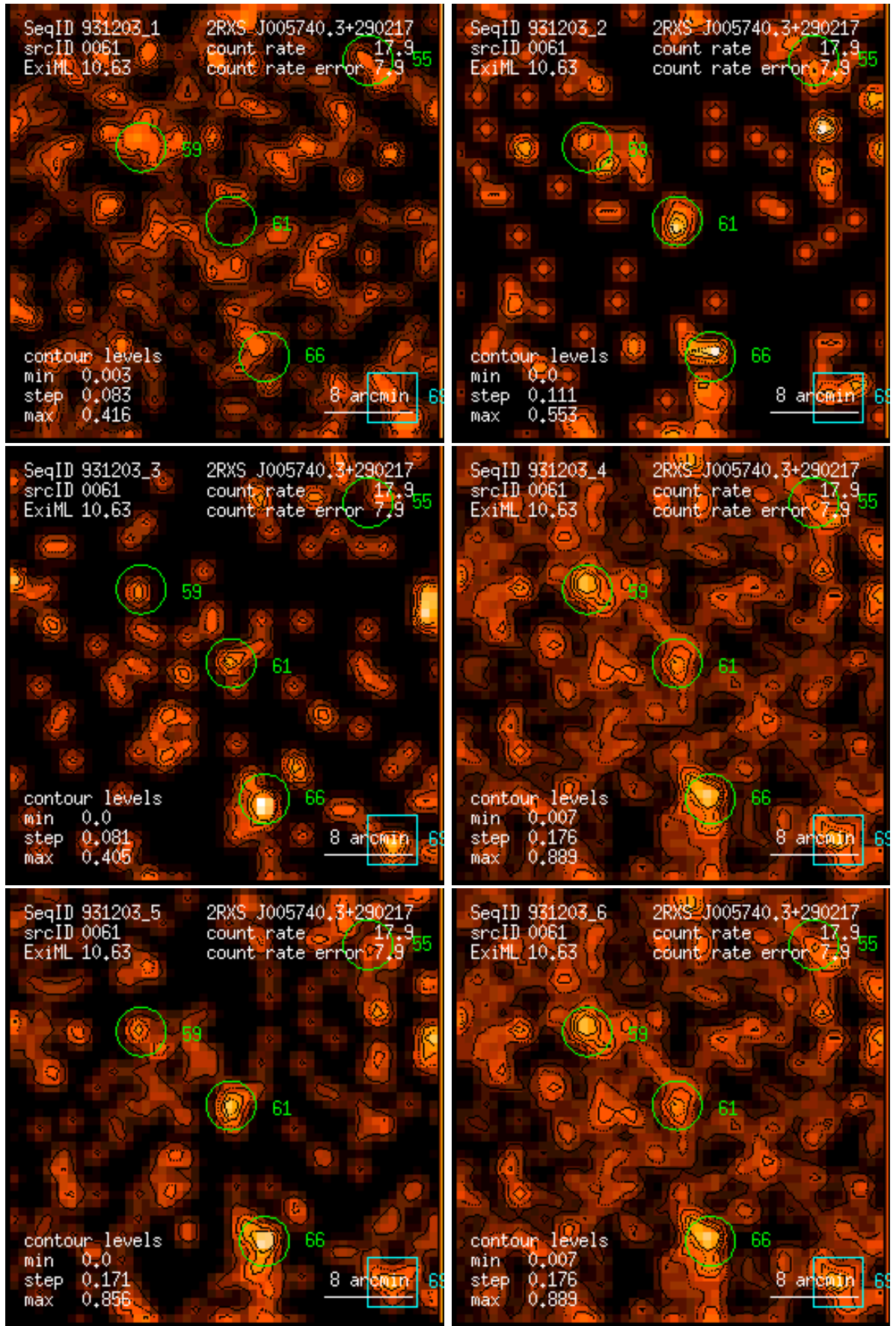
Figure 61: RASS 931203: detection 0061: band rate images, Gaussian filter: (1) PSPC channels 11 – 41, (2) 52 – 90, (3) 91 – 201, (4) 11 – 235, (5) 52 – 201, (6) 11 – 201. Broad band rates in counts/ks. Band rate contour levels in counts/ks/arcmin 2 .
