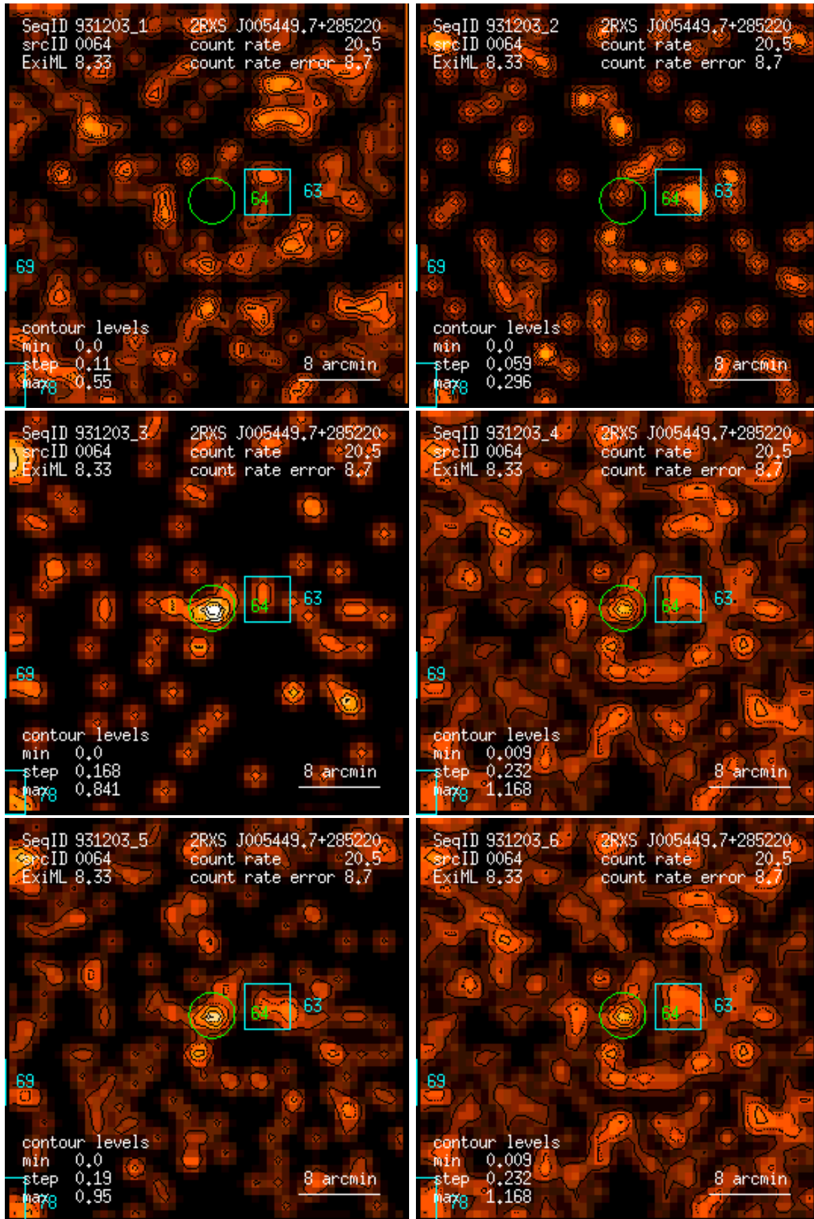
Figure 64: RASS 931203: detection 0064: band rate images, Gaussian filter: (1) PSPC channels 11 – 41, (2) 52 – 90, (3) 91 – 201, (4) 11 – 235, (5) 52 – 201, (6) 11 – 201. Broad band rates in counts/ks. Band rate contour levels in counts/ks/arcmin 2 .
