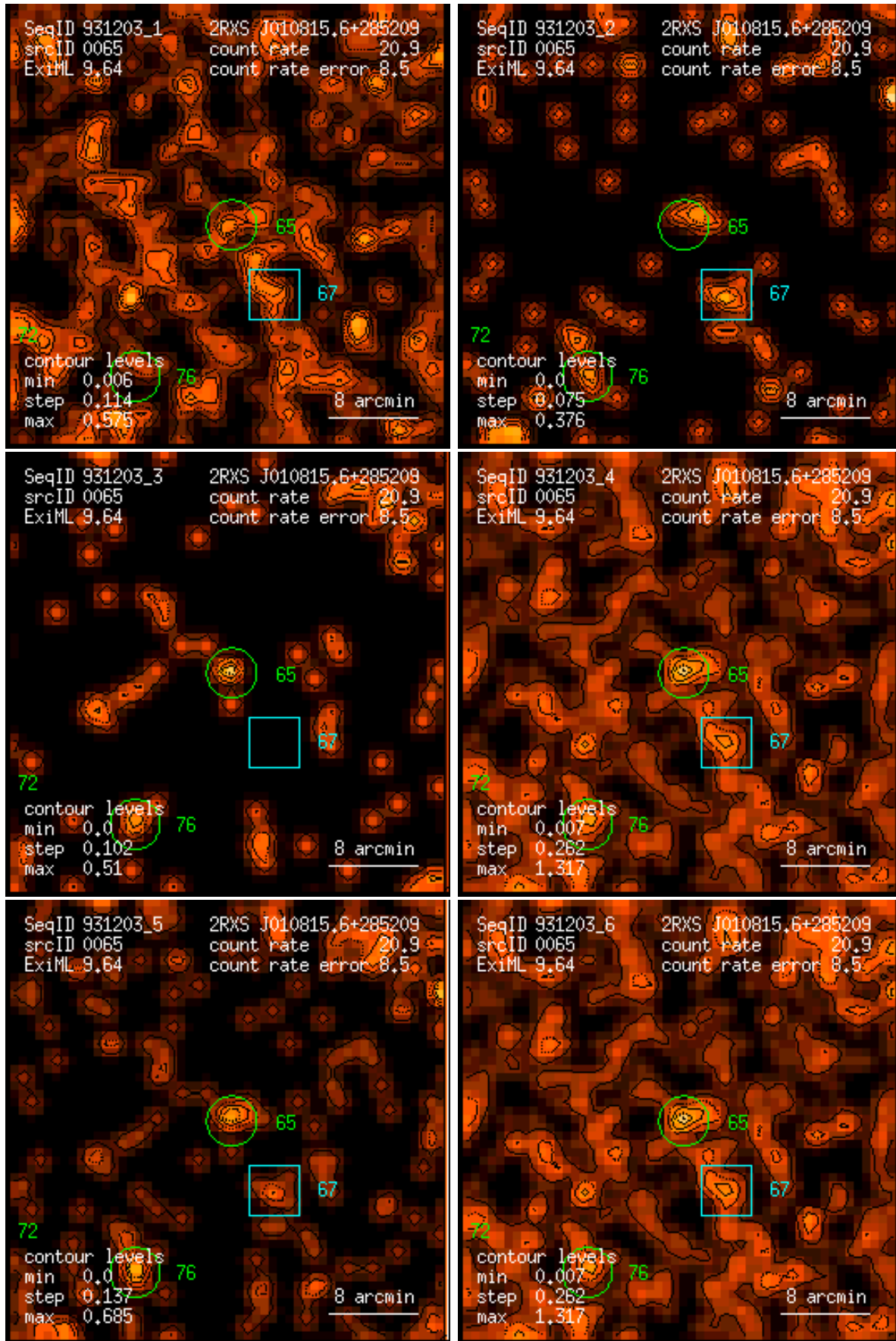
Figure 65: RASS 931203: detection 0065: band rate images, Gaussian filter: (1) PSPC channels 11 – 41, (2) 52 – 90, (3) 91 – 201, (4) 11 – 235, (5) 52 – 201, (6) 11 – 201. Broad band rates in counts/ks. Band rate contour levels in counts/ks/arcmin 2 .
