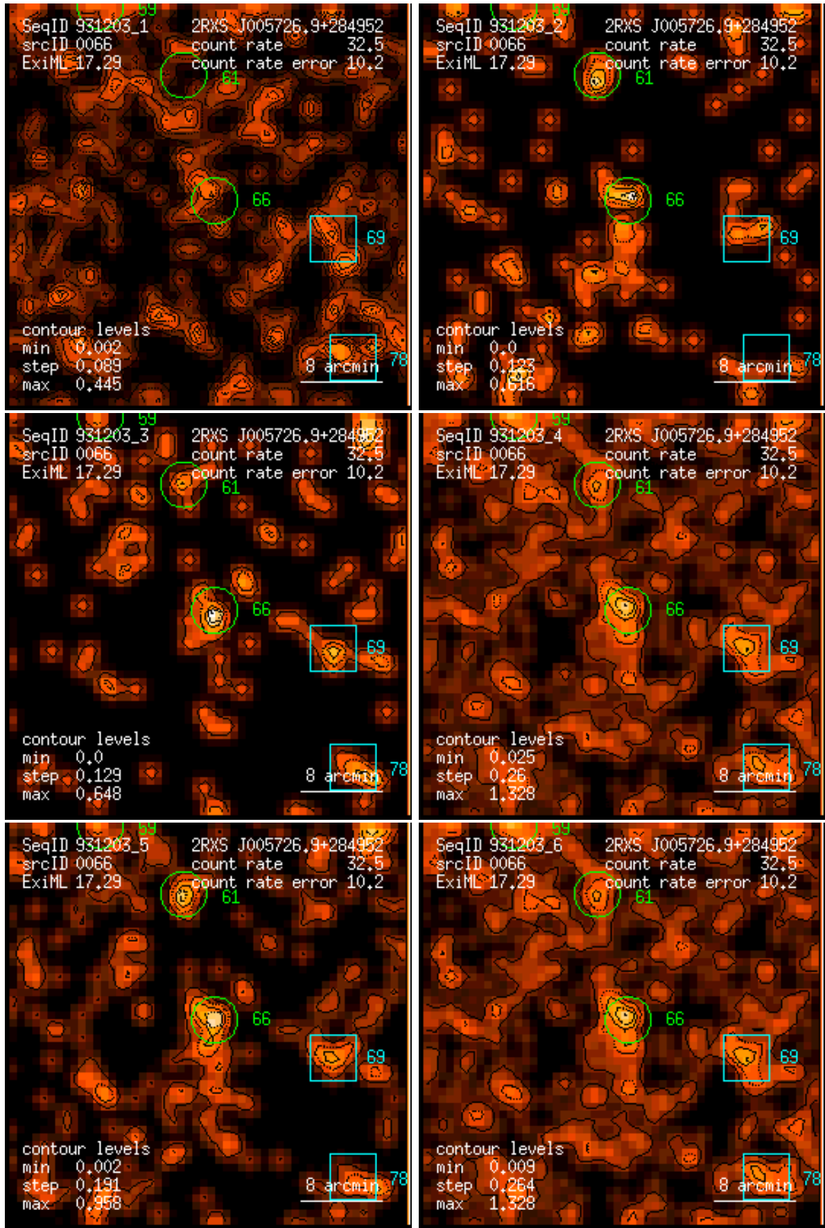
Figure 66: RASS 931203: detection 0066: band rate images, Gaussian filter: (1) PSPC channels 11 – 41, (2) 52 – 90, (3) 91 – 201, (4) 11 – 235, (5) 52 – 201, (6) 11 – 201. Broad band rates in counts/ks. Band rate contour levels in counts/ks/arcmin 2 .
