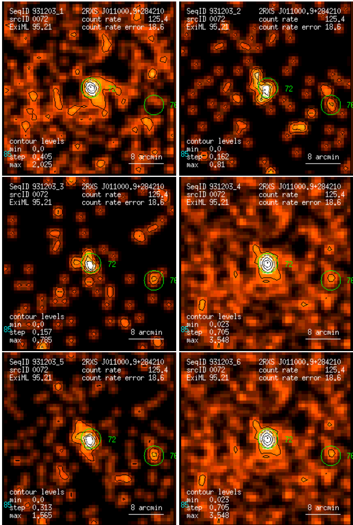
Figure 72: RASS 931203: detection 0072: band rate images, Gaussian filter: (1) PSPC channels 11 – 41, (2) 52 – 90, (3) 91 – 201, (4) 11 – 235, (5) 52 – 201, (6) 11 – 201. Broad band rates in counts/ks. Band rate contour levels in counts/ks/arcmin 2 .
