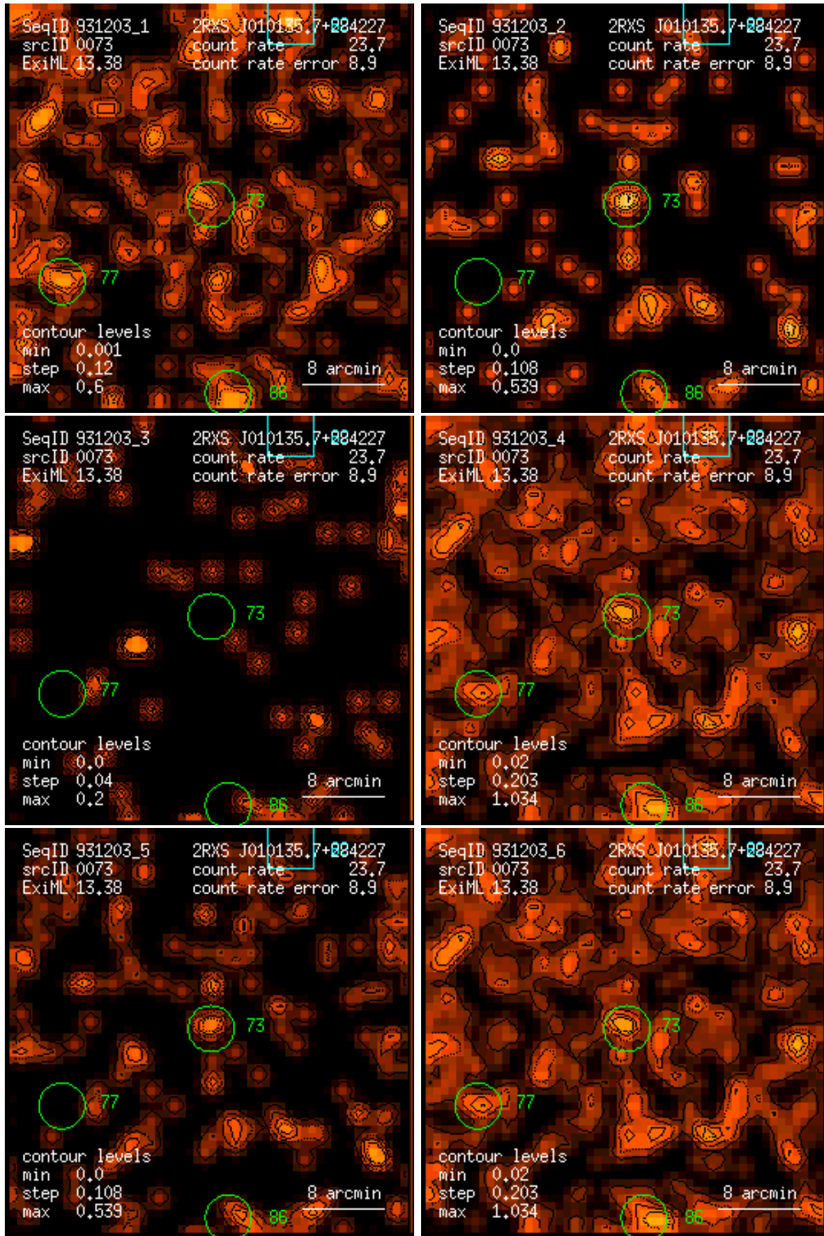
Figure 73: RASS 931203: detection 0073: band rate images, Gaussian filter: (1) PSPC channels 11 – 41, (2) 52 – 90, (3) 91 – 201, (4) 11 – 235, (5) 52 – 201, (6) 11 – 201. Broad band rates in counts/ks. Band rate contour levels in counts/ks/arcmin 2 .
