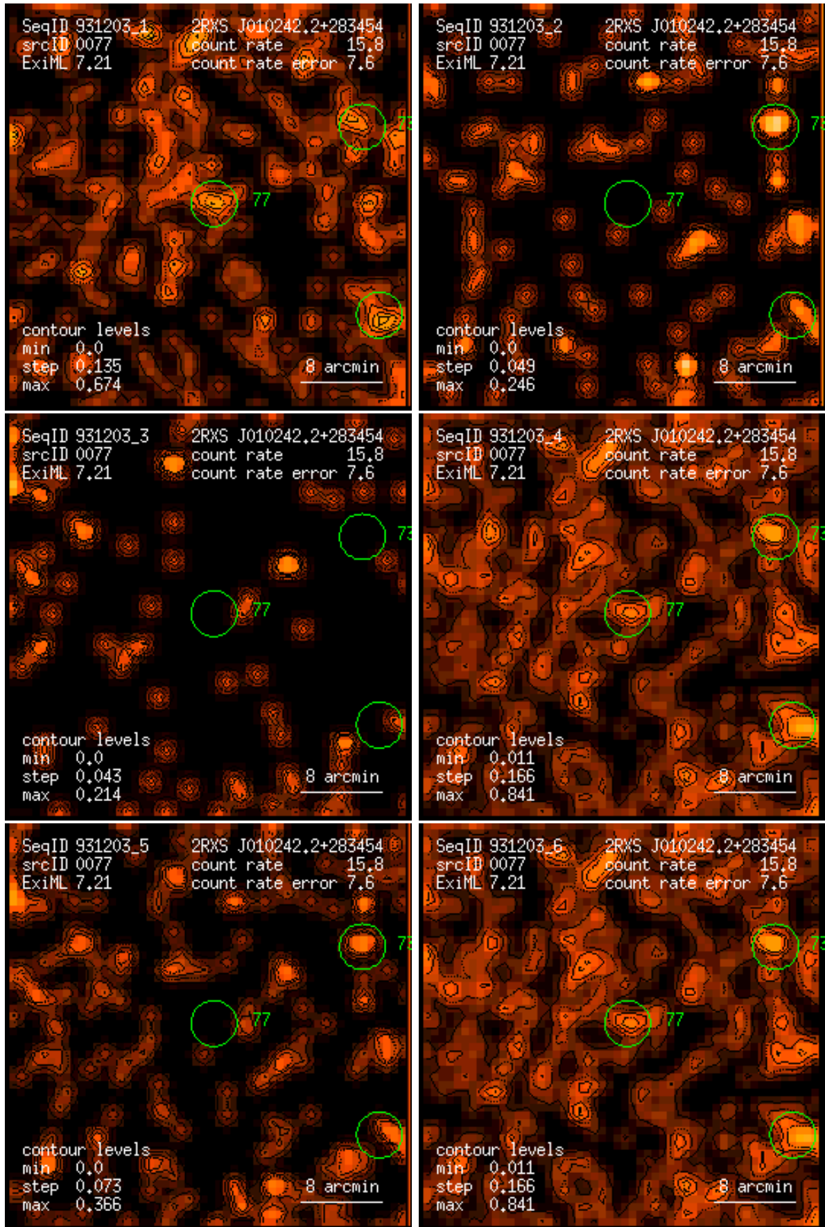
Figure 77: RASS 931203: detection 0077: band rate images, Gaussian filter: (1) PSPC channels 11 – 41, (2) 52 – 90, (3) 91 – 201, (4) 11 – 235, (5) 52 – 201, (6) 11 – 201. Broad band rates in counts/ks. Band rate contour levels in counts/ks/arcmin 2 .
