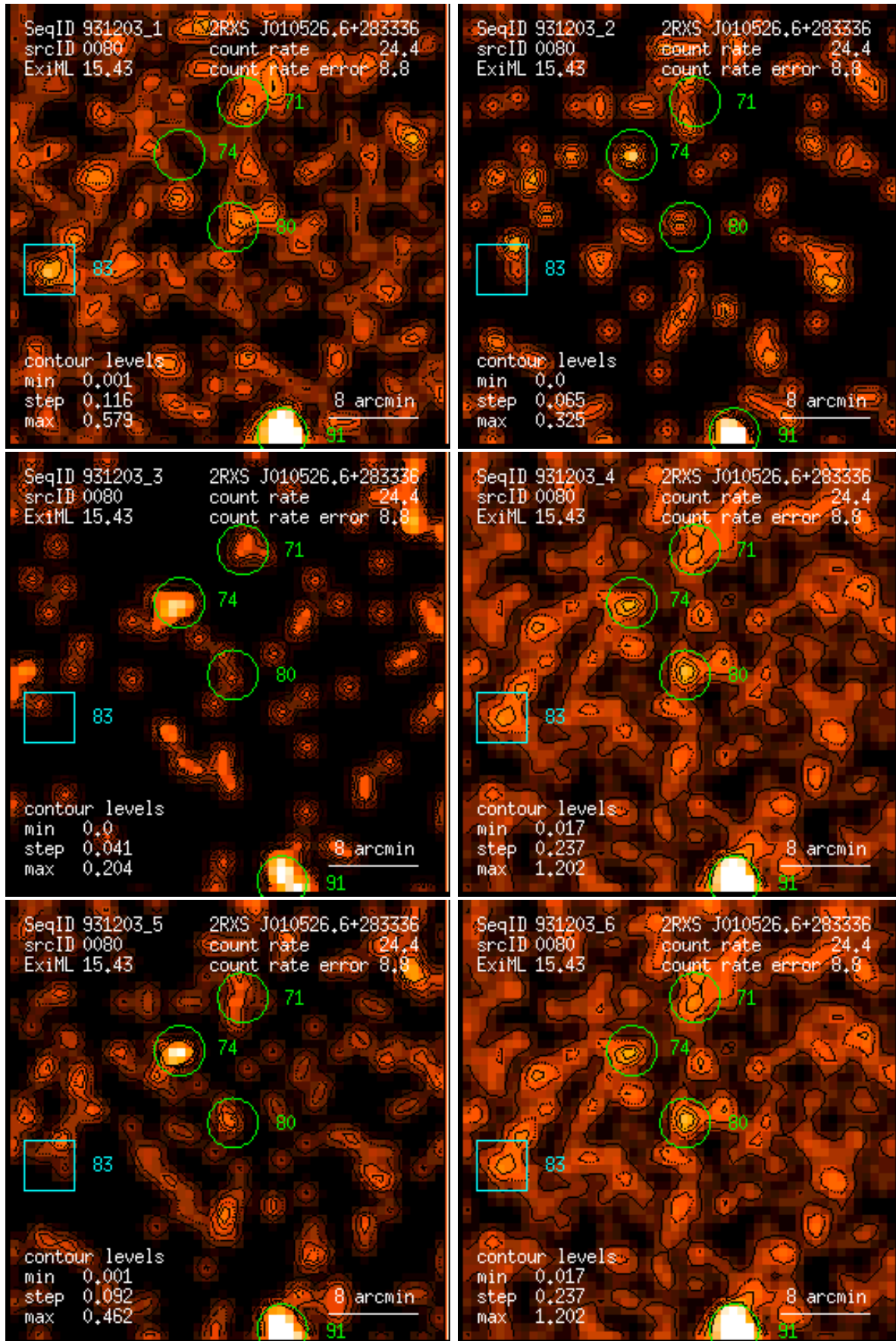
Figure 80: RASS 931203: detection 0080: band rate images, Gaussian filter: (1) PSPC channels 11 – 41, (2) 52 – 90, (3) 91 – 201, (4) 11 – 235, (5) 52 – 201, (6) 11 – 201. Broad band rates in counts/ks. Band rate contour levels in counts/ks/arcmin 2 .
