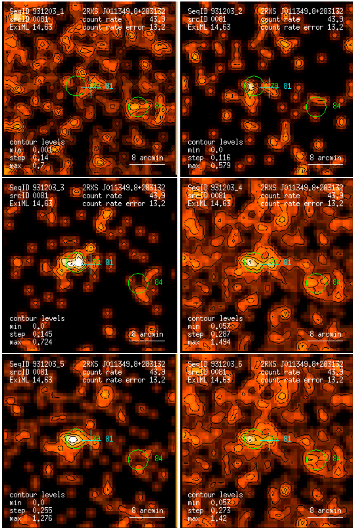
Figure 81: RASS 931203: detection 0081: band rate images, Gaussian filter: (1) PSPC channels 11 – 41, (2) 52 – 90, (3) 91 – 201, (4) 11 – 235, (5) 52 – 201, (6) 11 – 201. Broad band rates in counts/ks. Band rate contour levels in counts/ks/arcmin 2 .
