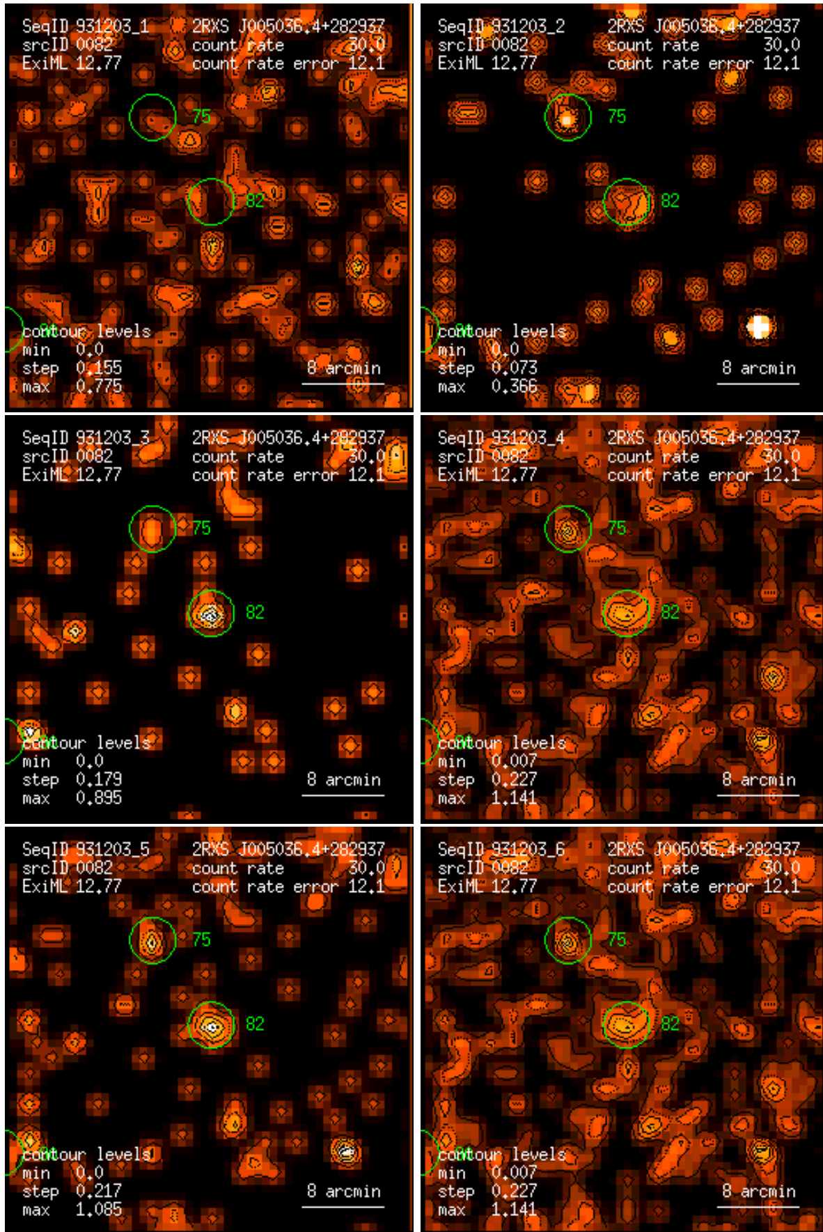
Figure 82: RASS 931203: detection 0082: band rate images, Gaussian filter: (1) PSPC channels 11 – 41, (2) 52 – 90, (3) 91 – 201, (4) 11 – 235, (5) 52 – 201, (6) 11 – 201. Broad band rates in counts/ks. Band rate contour levels in counts/ks/arcmin 2 .
