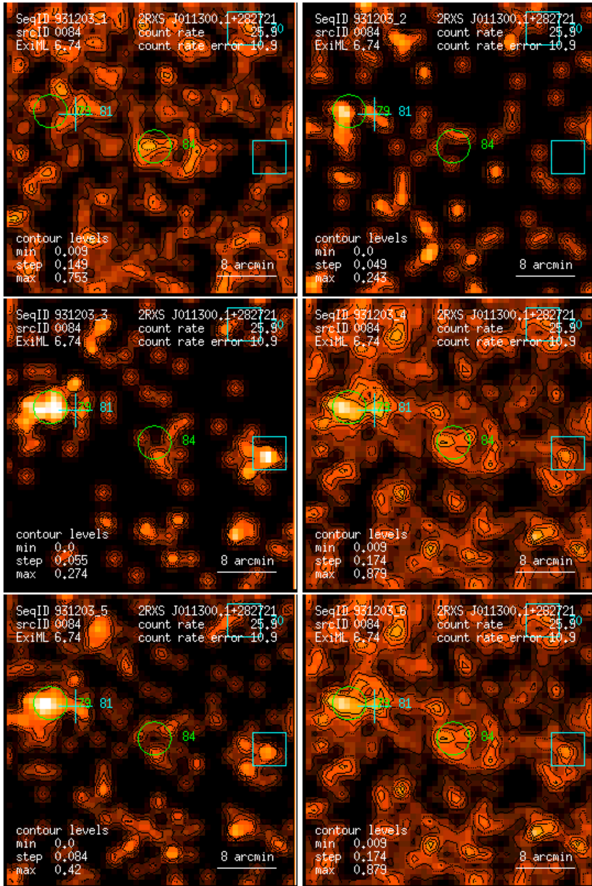
Figure 84: RASS 931203: detection 0084: band rate images, Gaussian filter: (1) PSPC channels 11 – 41, (2) 52 – 90, (3) 91 – 201, (4) 11 – 235, (5) 52 – 201, (6) 11 – 201. Broad band rates in counts/ks. Band rate contour levels in counts/ks/arcmin 2 .
