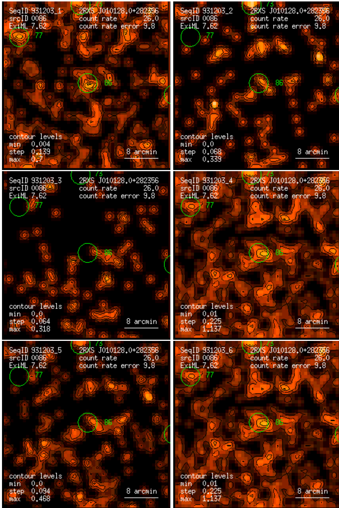
Figure 86: RASS 931203: detection 0086: band rate images, Gaussian filter: (1) PSPC channels 11 – 41, (2) 52 – 90, (3) 91 – 201, (4) 11 – 235, (5) 52 – 201, (6) 11 – 201. Broad band rates in counts/ks. Band rate contour levels in counts/ks/arcmin 2 .
