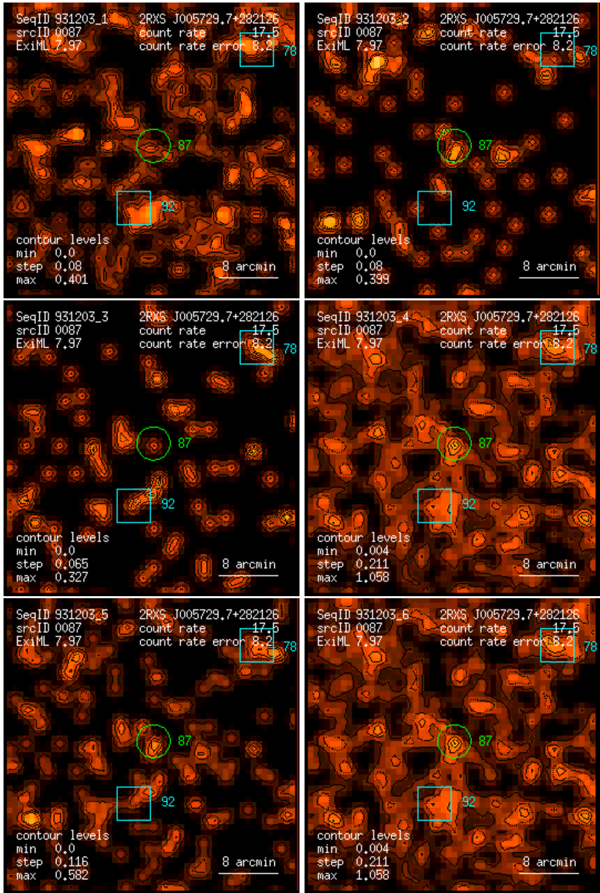
Figure 87: RASS 931203: detection 0087: band rate images, Gaussian filter: (1) PSPC channels 11 – 41, (2) 52 – 90, (3) 91 – 201, (4) 11 – 235, (5) 52 – 201, (6) 11 – 201. Broad band rates in counts/ks. Band rate contour levels in counts/ks/arcmin 2 .
