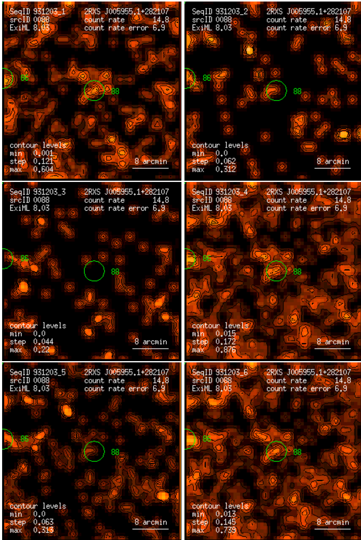
Figure 88: RASS 931203: detection 0088: band rate images, Gaussian filter: (1) PSPC channels 11 – 41, (2) 52 – 90, (3) 91 – 201, (4) 11 – 235, (5) 52 – 201, (6) 11 – 201. Broad band rates in counts/ks. Band rate contour levels in counts/ks/arcmin 2 .
