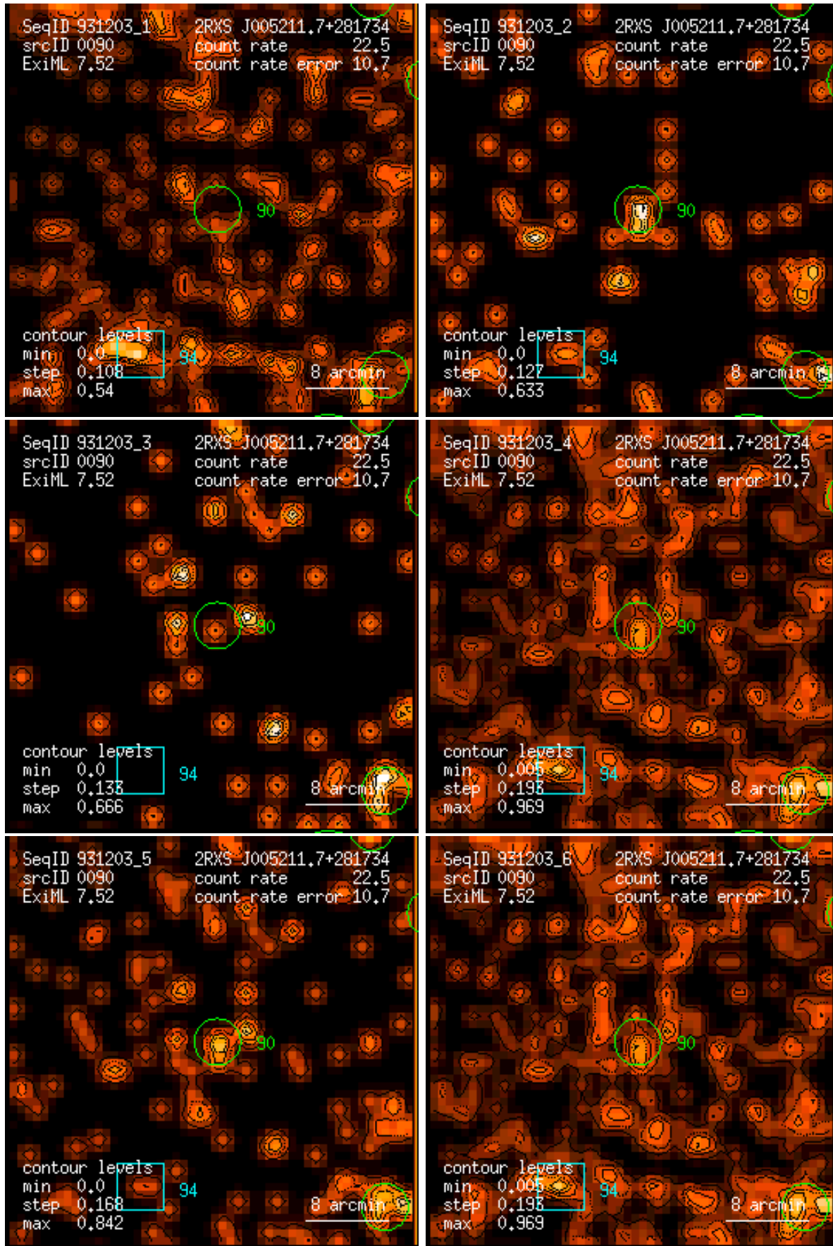
Figure 90: RASS 931203: detection 0090: band rate images, Gaussian filter: (1) PSPC channels 11 – 41, (2) 52 – 90, (3) 91 – 201, (4) 11 – 235, (5) 52 – 201, (6) 11 – 201. Broad band rates in counts/ks. Band rate contour levels in counts/ks/arcmin 2 .
