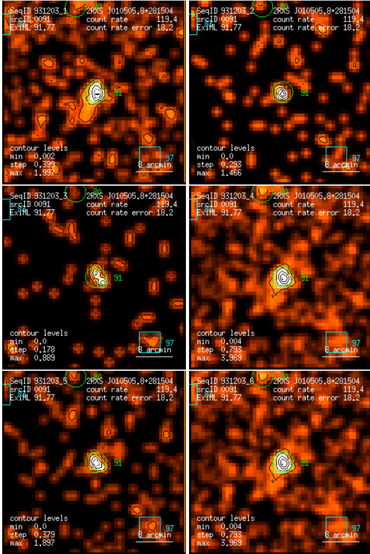
Figure 91: RASS 931203: detection 0091: band rate images, Gaussian filter: (1) PSPC channels 11 – 41, (2) 52 – 90, (3) 91 – 201, (4) 11 – 235, (5) 52 – 201, (6) 11 – 201. Broad band rates in counts/ks. Band rate contour levels in counts/ks/arcmin 2 .
