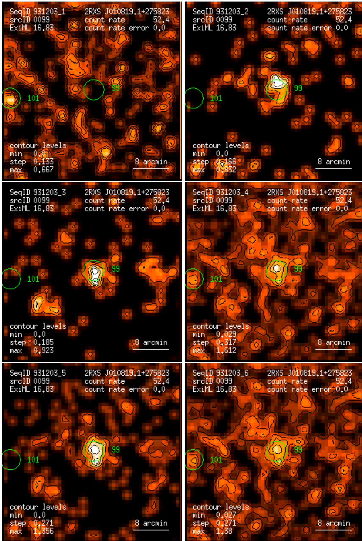
Figure 99: RASS 931203: detection 0099: band rate images, Gaussian filter: (1) PSPC channels 11 – 41, (2) 52 – 90, (3) 91 – 201, (4) 11 – 235, (5) 52 – 201, (6) 11 – 201. Broad band rates in counts/ks. Band rate contour levels in counts/ks/arcmin 2 .
