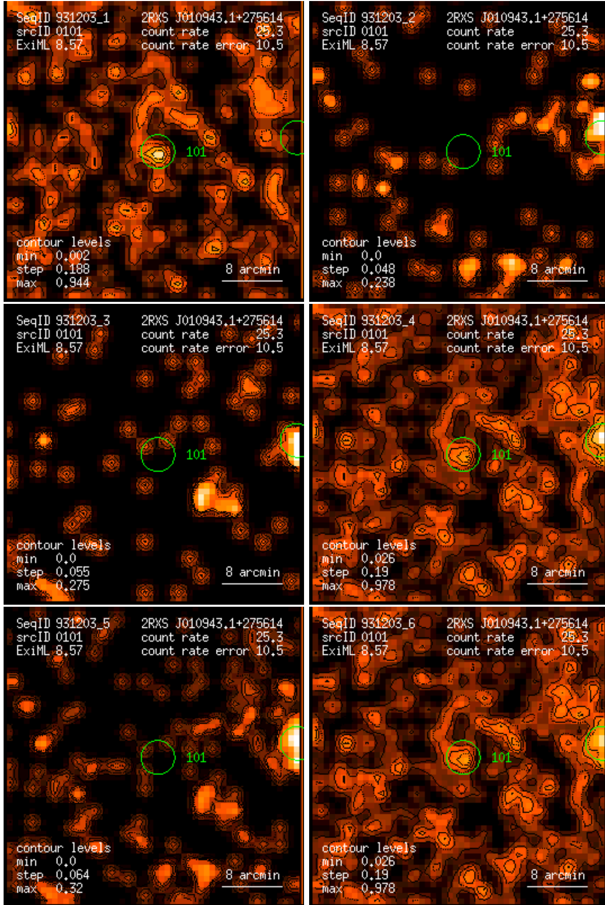
Figure 101: RASS 931203: detection 0101: band rate images, Gaussian filter: (1) PSPC channels 11 – 41, (2) 52 – 90, (3) 91 – 201, (4) 11 – 235, (5) 52 – 201, (6) 11 – 201. Broad band rates in counts/ks. Band rate contour levels in counts/ks/arcmin 2 .
