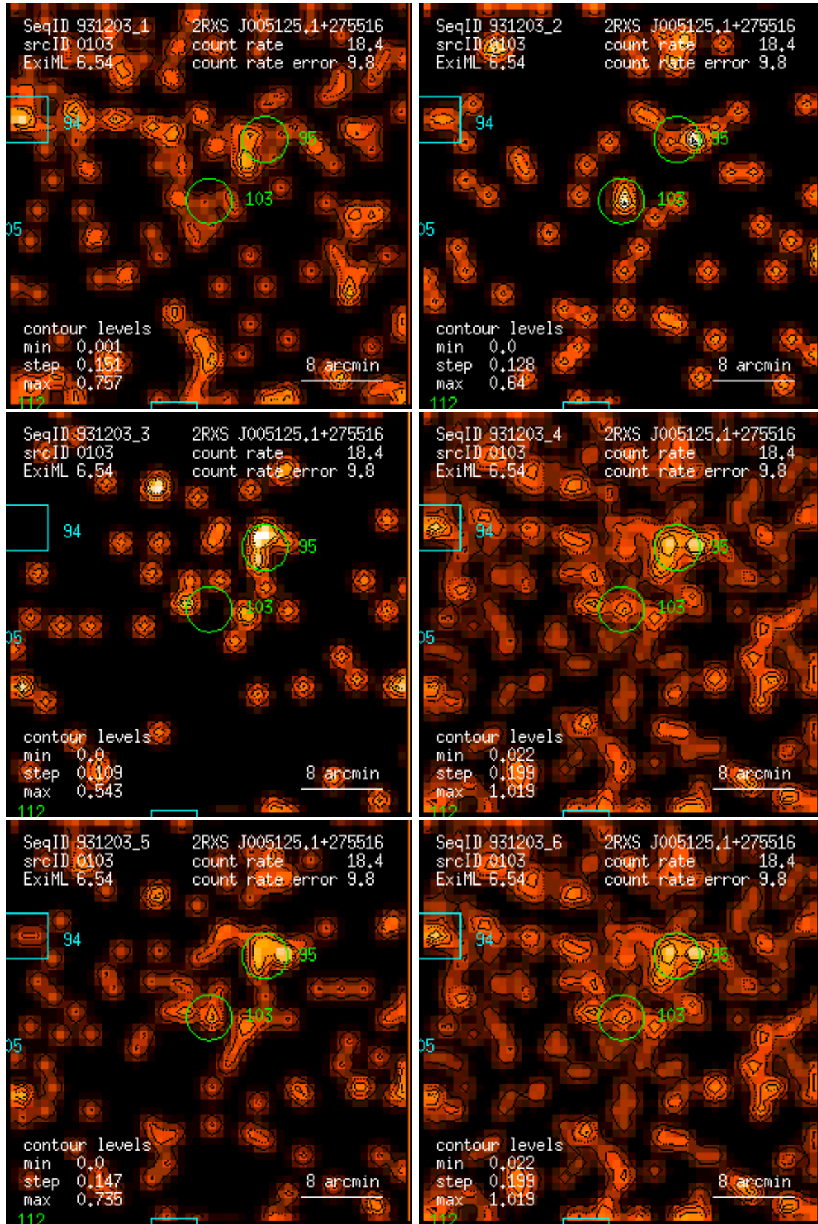
Figure 103: RASS 931203: detection 0103: band rate images, Gaussian filter: (1) PSPC channels 11 – 41, (2) 52 – 90, (3) 91 – 201, (4) 11 – 235, (5) 52 – 201, (6) 11 – 201. Broad band rates in counts/ks. Band rate contour levels in counts/ks/arcmin 2 .
