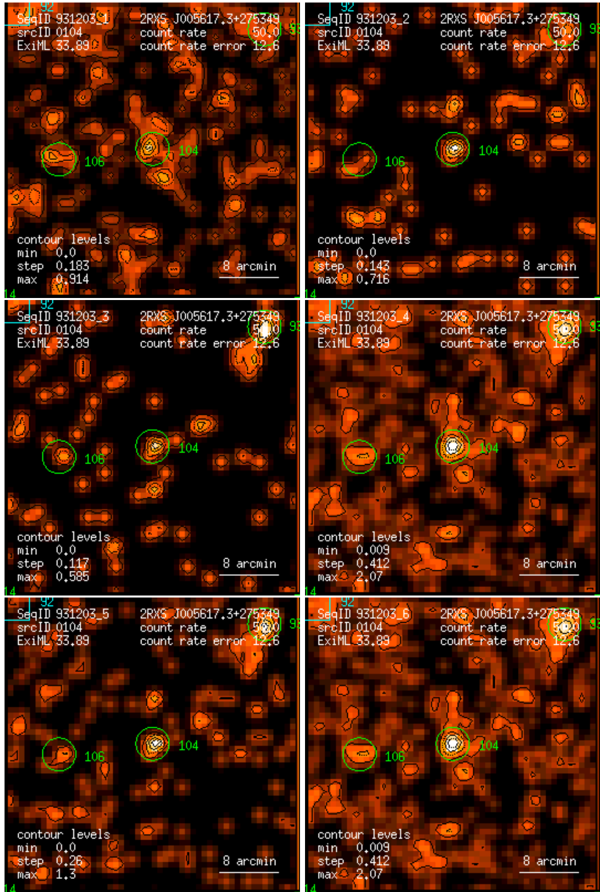
Figure 104: RASS 931203: detection 0104: band rate images, Gaussian filter: (1) PSPC channels 11 – 41, (2) 52 – 90, (3) 91 – 201, (4) 11 – 235, (5) 52 – 201, (6) 11 – 201. Broad band rates in counts/ks. Band rate contour levels in counts/ks/arcmin 2 .
