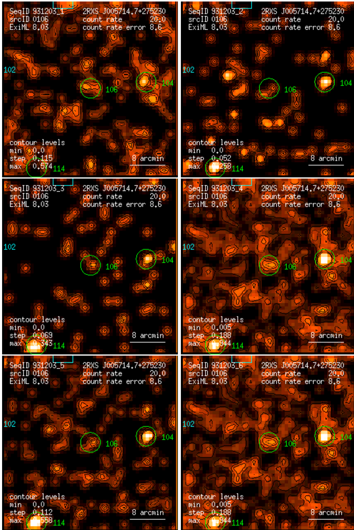
Figure 106: RASS 931203: detection 0106: band rate images, Gaussian filter: (1) PSPC channels 11 – 41, (2) 52 – 90, (3) 91 – 201, (4) 11 – 235, (5) 52 – 201, (6) 11 – 201. Broad band rates in counts/ks. Band rate contour levels in counts/ks/arcmin 2 .
