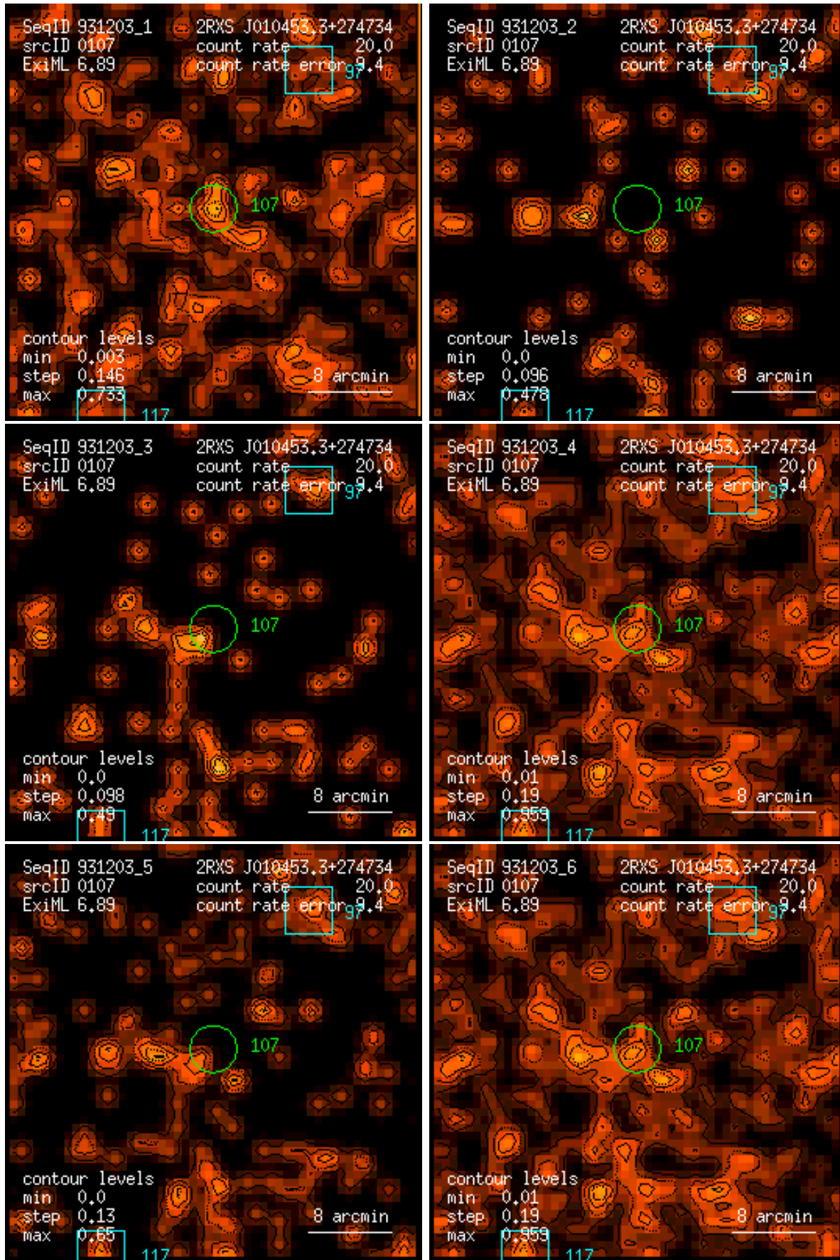
Figure 107: RASS 931203: detection 0107: band rate images, Gaussian filter: (1) PSPC channels 11 – 41, (2) 52 – 90, (3) 91 – 201, (4) 11 – 235, (5) 52 – 201, (6) 11 – 201. Broad band rates in counts/ks. Band rate contour levels in counts/ks/arcmin 2 .
