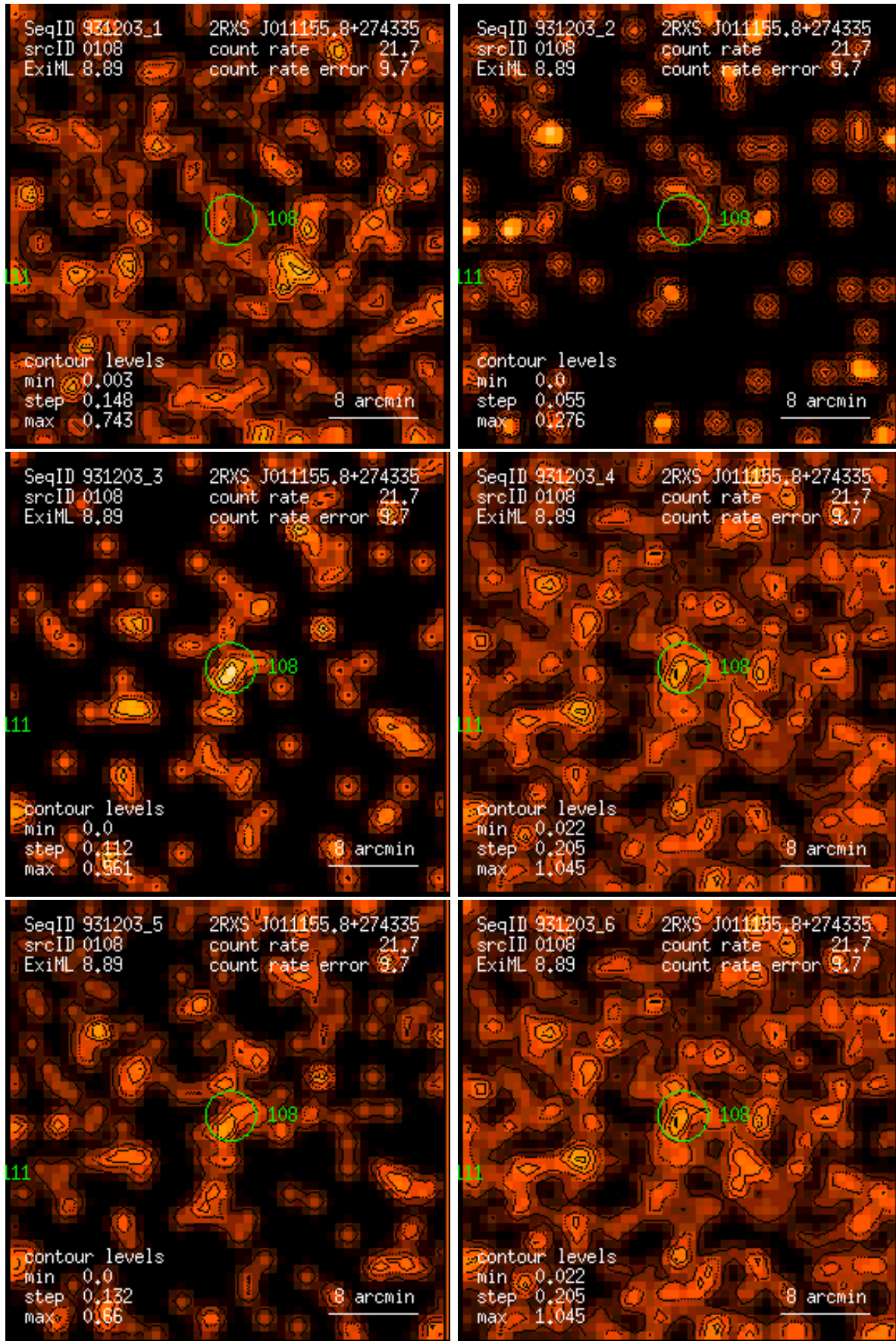
Figure 108: RASS 931203: detection 0108: band rate images, Gaussian filter: (1) PSPC channels 11 – 41, (2) 52 – 90, (3) 91 – 201, (4) 11 – 235, (5) 52 – 201, (6) 11 – 201. Broad band rates in counts/ks. Band rate contour levels in counts/ks/arcmin 2 .
