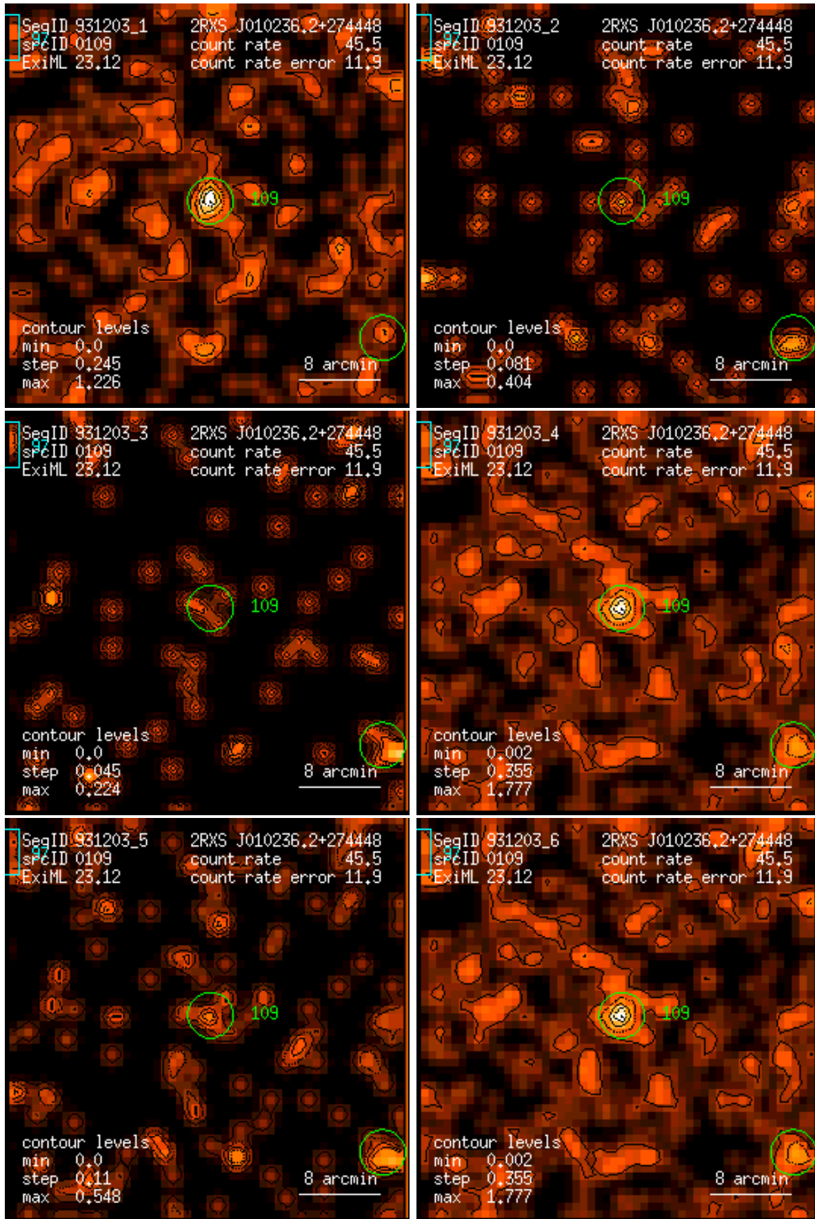
Figure 109: RASS 931203: detection 0109: band rate images, Gaussian filter: (1) PSPC channels 11 – 41, (2) 52 – 90, (3) 91 – 201, (4) 11 – 235, (5) 52 – 201, (6) 11 – 201. Broad band rates in counts/ks. Band rate contour levels in counts/ks/arcmin 2 .
