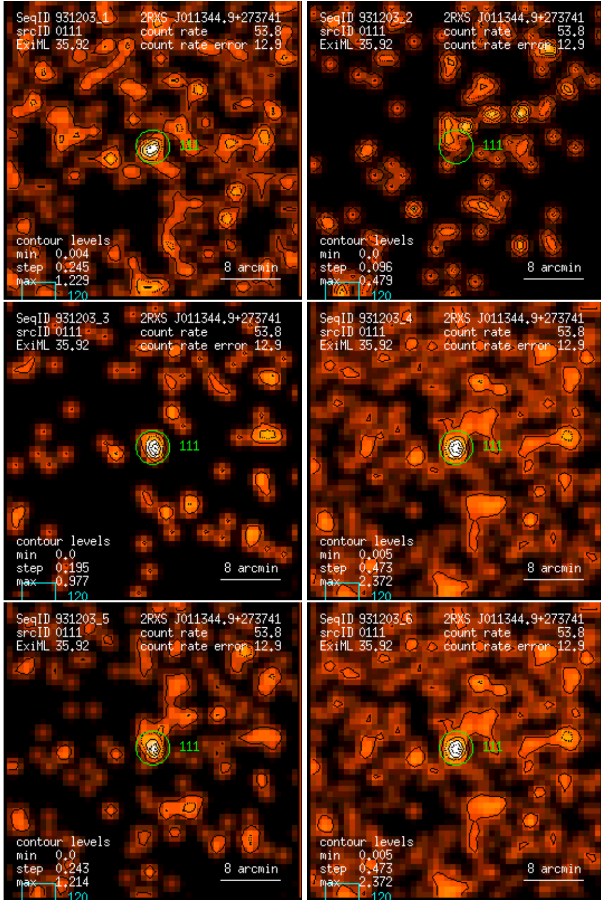
Figure 111: RASS 931203: detection 0111: band rate images, Gaussian filter: (1) PSPC channels 11 – 41, (2) 52 – 90, (3) 91 – 201, (4) 11 – 235, (5) 52 – 201, (6) 11 – 201. Broad band rates in counts/ks. Band rate contour levels in counts/ks/arcmin 2 .
