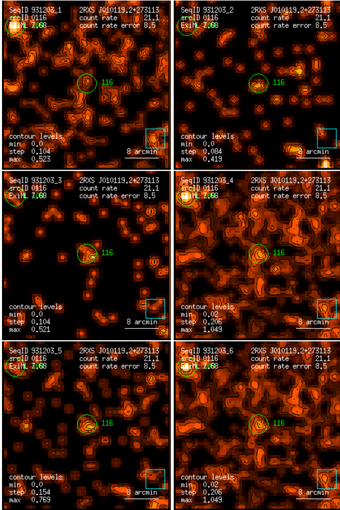
Figure 116: RASS 931203: detection 0116: band rate images, Gaussian filter: (1) PSPC channels 11 – 41, (2) 52 – 90, (3) 91 – 201, (4) 11 – 235, (5) 52 – 201, (6) 11 – 201. Broad band rates in counts/ks. Band rate contour levels in counts/ks/arcmin 2 .
