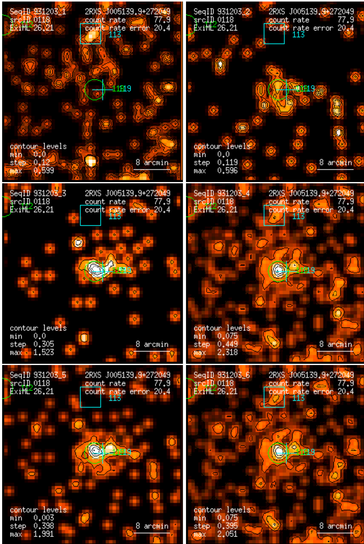
Figure 118: RASS 931203: detection 0118: band rate images, Gaussian filter: (1) PSPC channels 11 – 41, (2) 52 – 90, (3) 91 – 201, (4) 11 – 235, (5) 52 – 201, (6) 11 – 201. Broad band rates in counts/ks. Band rate contour levels in counts/ks/arcmin 2 .
