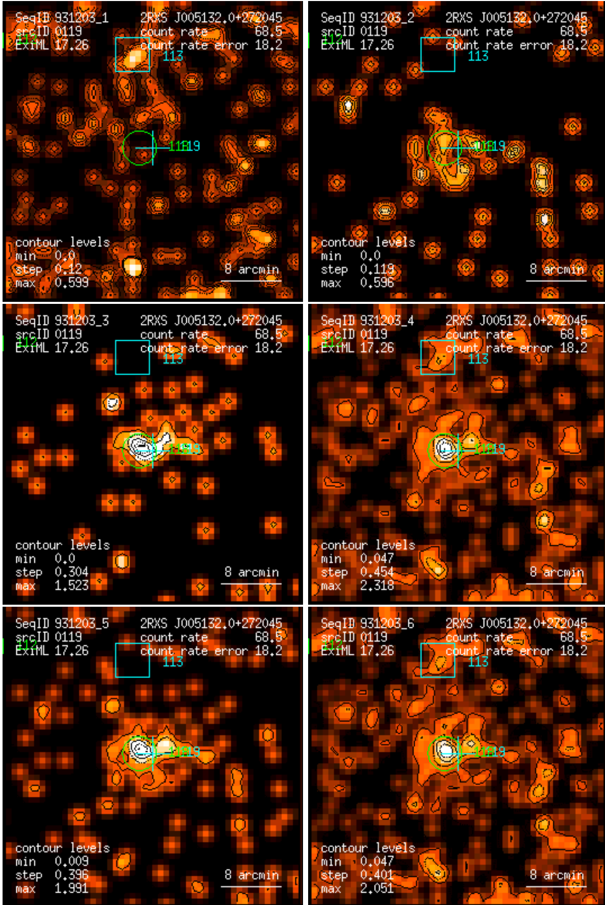
Figure 119: RASS 931203: detection 0119: band rate images, Gaussian filter: (1) PSPC channels 11 – 41, (2) 52 – 90, (3) 91 – 201, (4) 11 – 235, (5) 52 – 201, (6) 11 – 201. Broad band rates in counts/ks. Band rate contour levels in counts/ks/arcmin 2 .
