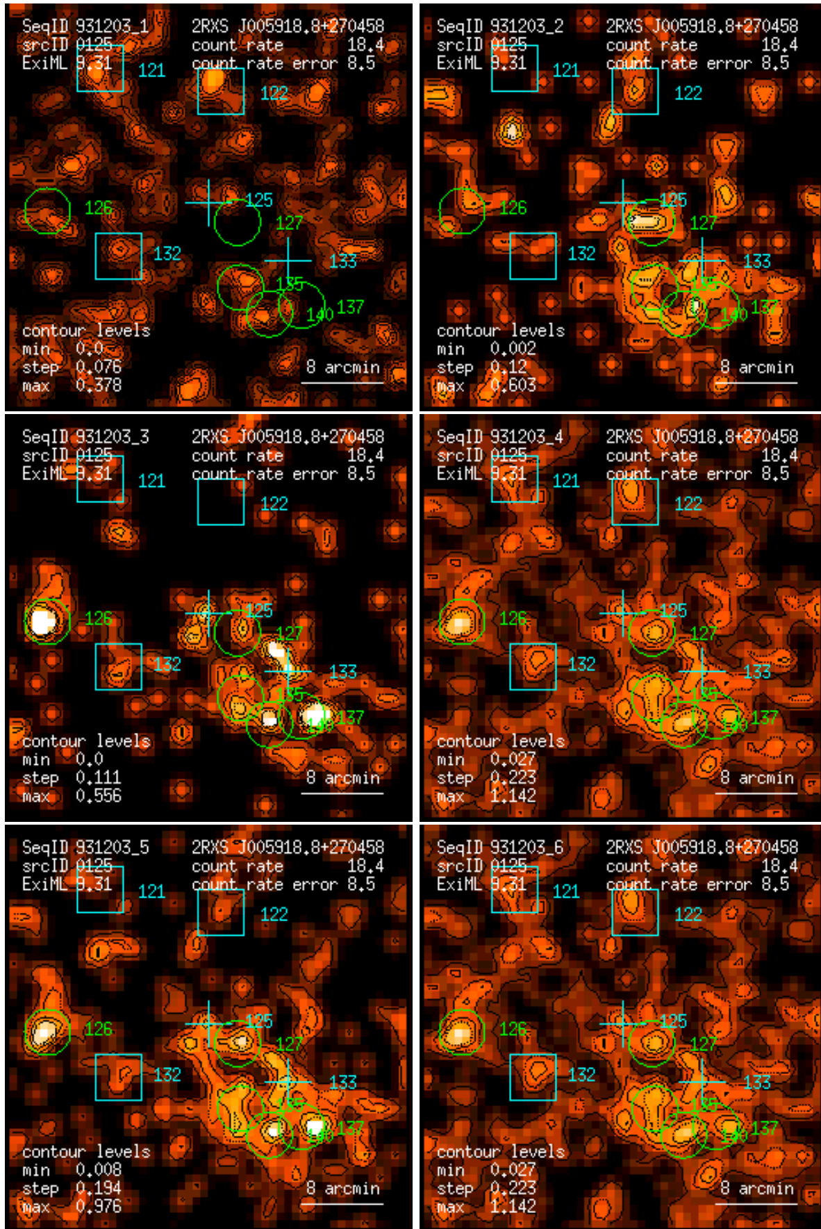
Figure 125: RASS 931203: detection 0125: band rate images, Gaussian filter: (1) PSPC channels 11 – 41, (2) 52 – 90, (3) 91 – 201, (4) 11 – 235, (5) 52 – 201, (6) 11 – 201. Broad band rates in counts/ks. Band rate contour levels in counts/ks/arcmin 2 .
