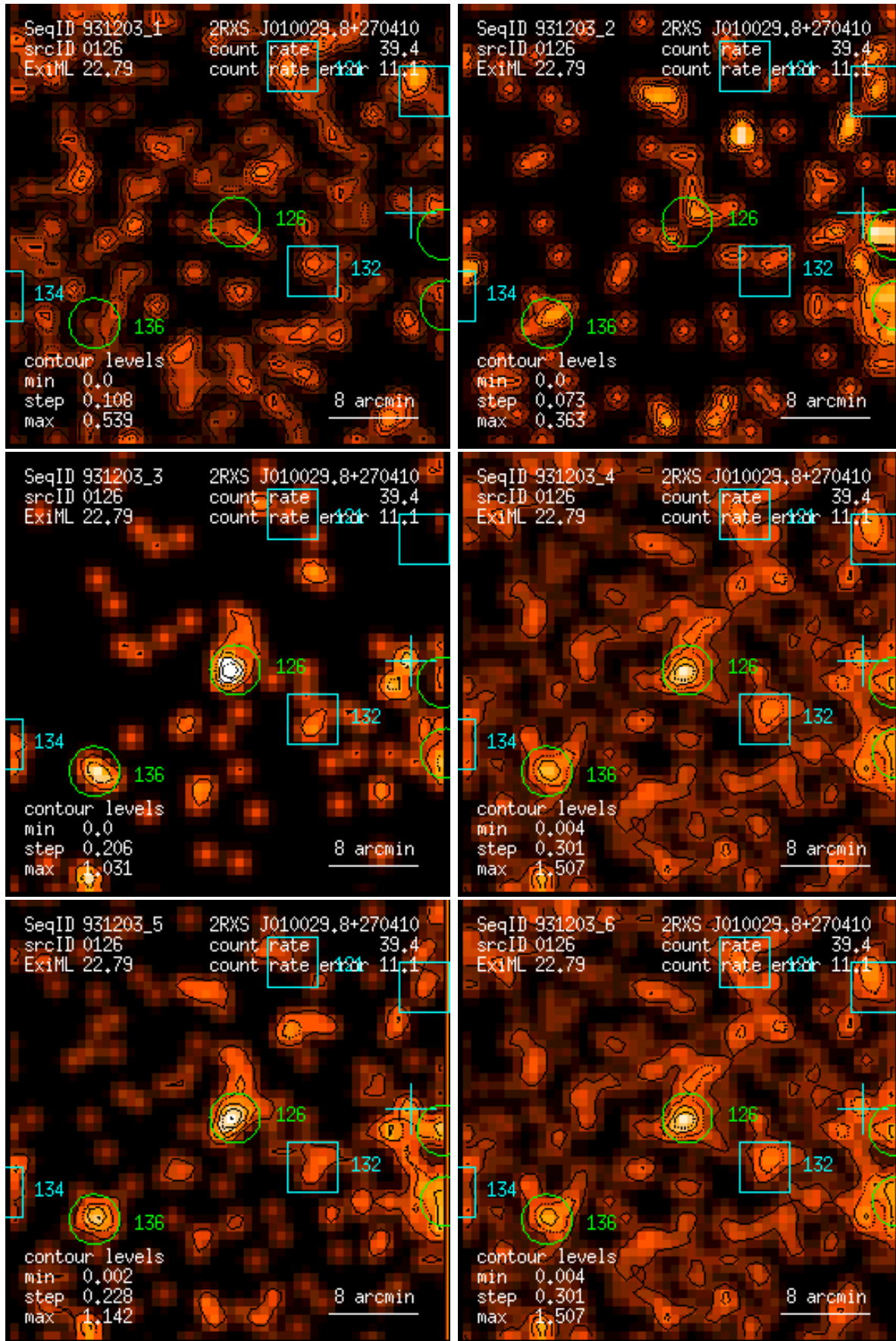
Figure 126: RASS 931203: detection 0126: band rate images, Gaussian filter: (1) PSPC channels 11 – 41, (2) 52 – 90, (3) 91 – 201, (4) 11 – 235, (5) 52 – 201, (6) 11 – 201. Broad band rates in counts/ks. Band rate contour levels in counts/ks/arcmin 2 .
