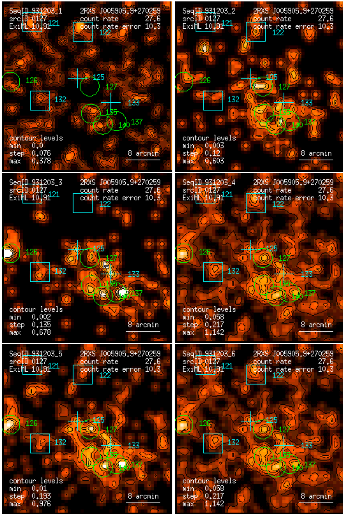
Figure 127: RASS 931203: detection 0127: band rate images, Gaussian filter: (1) PSPC channels 11 – 41, (2) 52 – 90, (3) 91 – 201, (4) 11 – 235, (5) 52 – 201, (6) 11 – 201. Broad band rates in counts/ks. Band rate contour levels in counts/ks/arcmin 2 .
