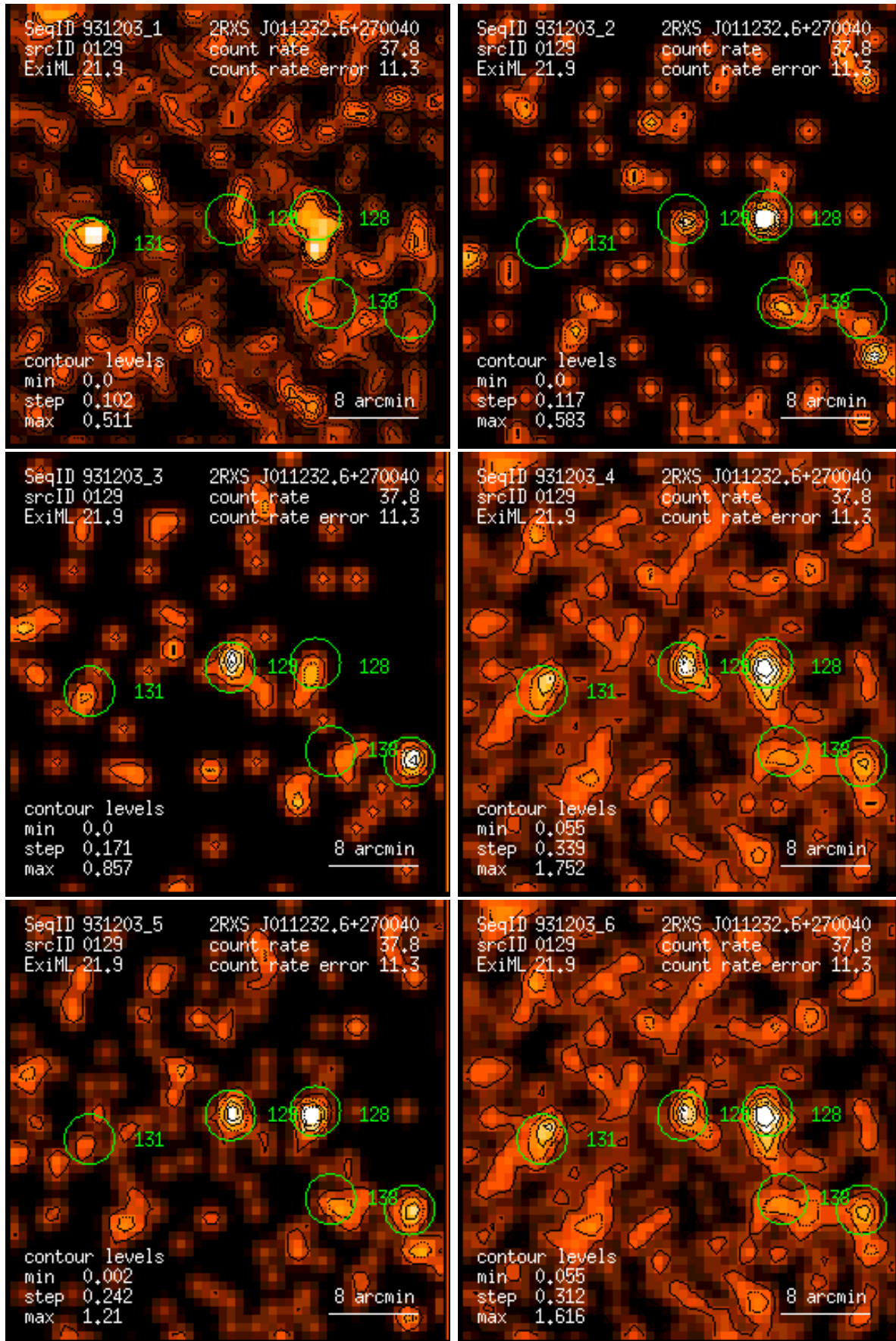
Figure 129: RASS 931203: detection 0129: band rate images, Gaussian filter: (1) PSPC channels 11 – 41, (2) 52 – 90, (3) 91 – 201, (4) 11 – 235, (5) 52 – 201, (6) 11 – 201. Broad band rates in counts/ks. Band rate contour levels in counts/ks/arcmin 2 .
