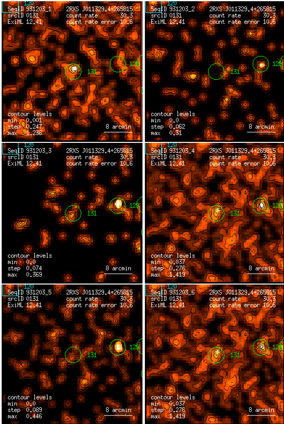
Figure 131: RASS 931203: detection 0131: band rate images, Gaussian filter: (1) PSPC channels 11 – 41, (2) 52 – 90, (3) 91 – 201, (4) 11 – 235, (5) 52 – 201, (6) 11 – 201. Broad band rates in counts/ks. Band rate contour levels in counts/ks/arcmin 2 .
