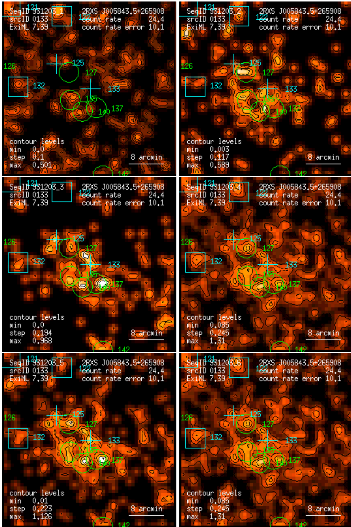
Figure 133: RASS 931203: detection 0133: band rate images, Gaussian filter: (1) PSPC channels 11 – 41, (2) 52 – 90, (3) 91 – 201, (4) 11 – 235, (5) 52 – 201, (6) 11 – 201. Broad band rates in counts/ks. Band rate contour levels in counts/ks/arcmin 2 .
