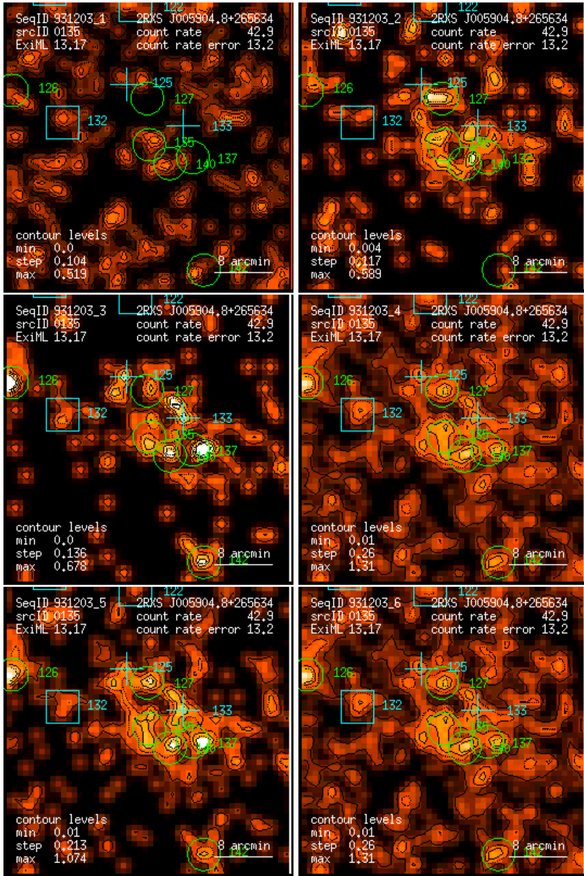
Figure 135: RASS 931203: detection 0135: band rate images, Gaussian filter: (1) PSPC channels 11 – 41, (2) 52 – 90, (3) 91 – 201, (4) 11 – 235, (5) 52 – 201, (6) 11 – 201. Broad band rates in counts/ks. Band rate contour levels in counts/ks/arcmin 2 .
