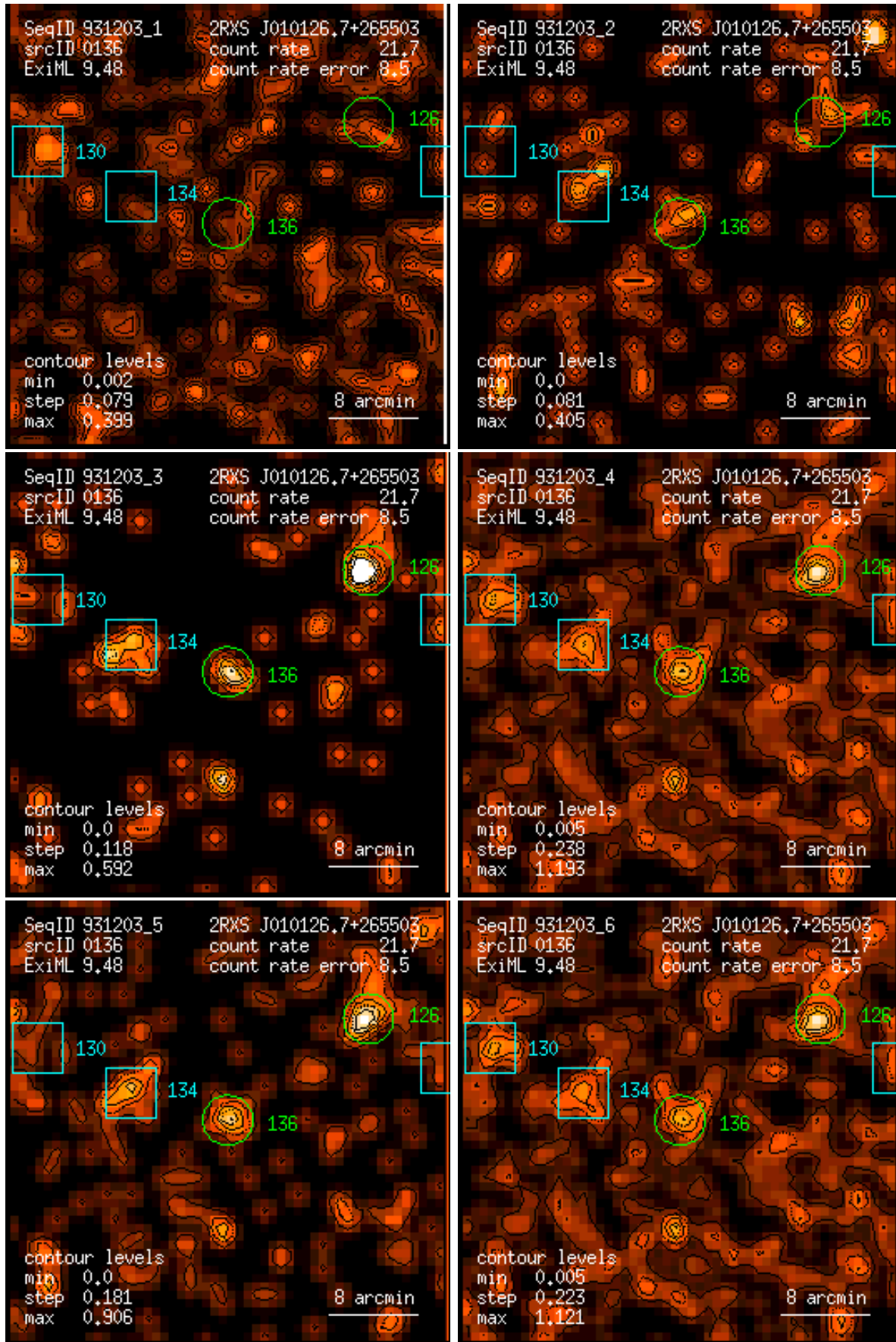
Figure 136: RASS 931203: detection 0136: band rate images, Gaussian filter: (1) PSPC channels 11 – 41, (2) 52 – 90, (3) 91 – 201, (4) 11 – 235, (5) 52 – 201, (6) 11 – 201. Broad band rates in counts/ks. Band rate contour levels in counts/ks/arcmin 2 .
