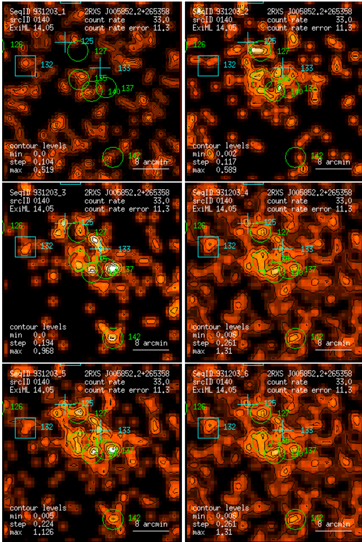
Figure 140: RASS 931203: detection 0140: band rate images, Gaussian filter: (1) PSPC channels 11 – 41, (2) 52 – 90, (3) 91 – 201, (4) 11 – 235, (5) 52 – 201, (6) 11 – 201. Broad band rates in counts/ks. Band rate contour levels in counts/ks/arcmin 2 .
