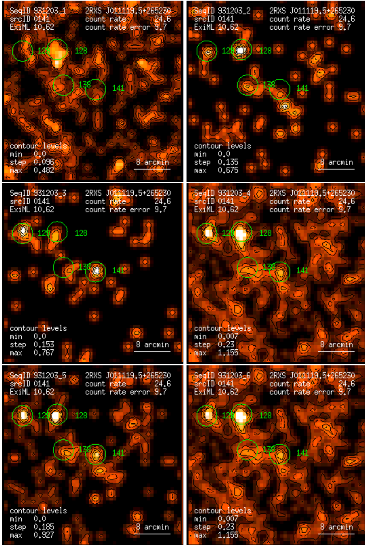
Figure 141: RASS 931203: detection 0141: band rate images, Gaussian filter: (1) PSPC channels 11 – 41, (2) 52 – 90, (3) 91 – 201, (4) 11 – 235, (5) 52 – 201, (6) 11 – 201. Broad band rates in counts/ks. Band rate contour levels in counts/ks/arcmin 2 .
