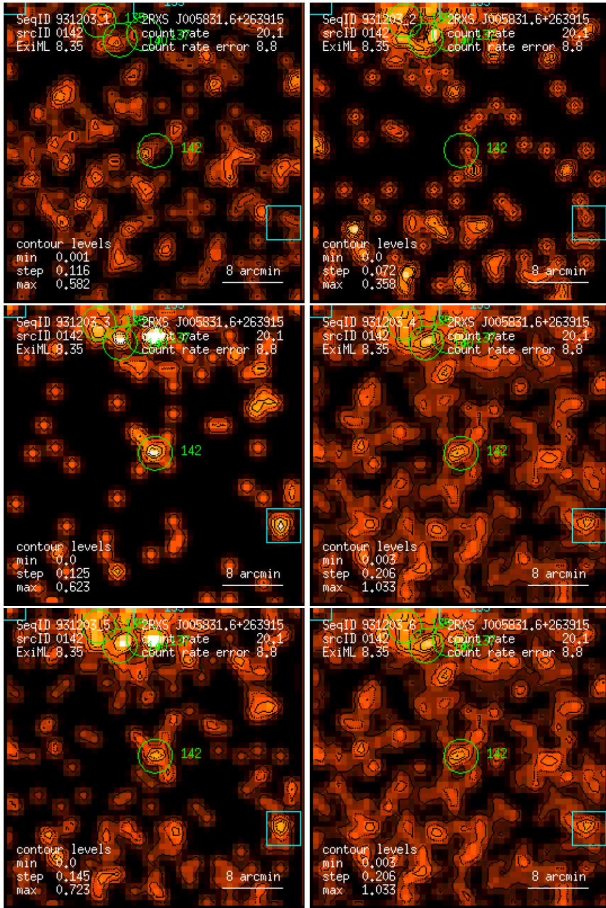
Figure 142: RASS 931203: detection 0142: band rate images, Gaussian filter: (1) PSPC channels 11 – 41, (2) 52 – 90, (3) 91 – 201, (4) 11 – 235, (5) 52 – 201, (6) 11 – 201. Broad band rates in counts/ks. Band rate contour levels in counts/ks/arcmin 2 .
