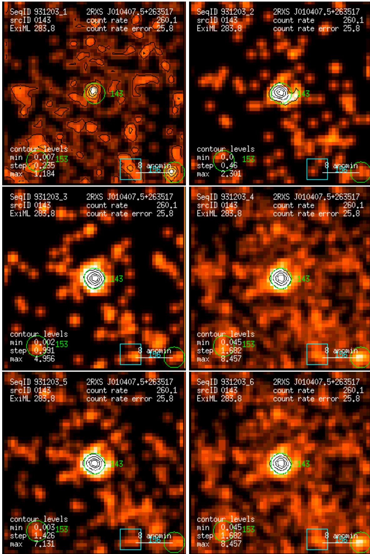
Figure 143: RASS 931203: detection 0143: band rate images, Gaussian filter: (1) PSPC channels 11 – 41, (2) 52 – 90, (3) 91 – 201, (4) 11 – 235, (5) 52 – 201, (6) 11 – 201. Broad band rates in counts/ks. Band rate contour levels in counts/ks/arcmin 2 .
