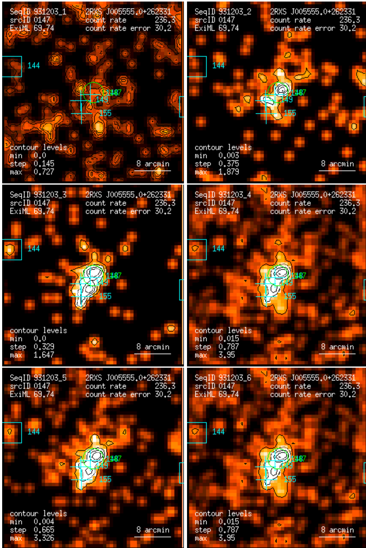
Figure 147: RASS 931203: detection 0147: band rate images, Gaussian filter: (1) PSPC channels 11 – 41, (2) 52 – 90, (3) 91 – 201, (4) 11 – 235, (5) 52 – 201, (6) 11 – 201. Broad band rates in counts/ks. Band rate contour levels in counts/ks/arcmin 2 .
