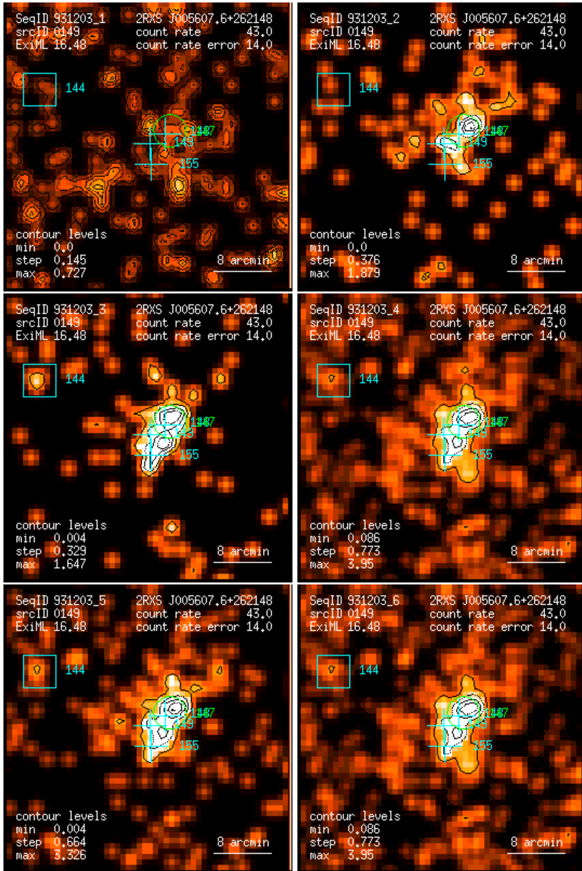
Figure 149: RASS 931203: detection 0149: band rate images, Gaussian filter: (1) PSPC channels 11 – 41, (2) 52 – 90, (3) 91 – 201, (4) 11 – 235, (5) 52 – 201, (6) 11 – 201. Broad band rates in counts/ks. Band rate contour levels in counts/ks/arcmin 2 .
