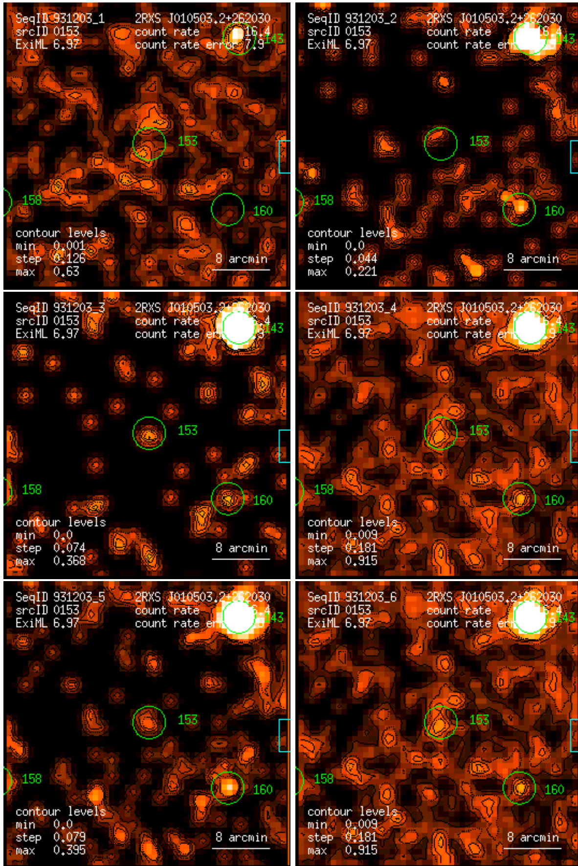
Figure 153: RASS 931203: detection 0153: band rate images, Gaussian filter: (1) PSPC channels 11 – 41, (2) 52 – 90, (3) 91 – 201, (4) 11 – 235, (5) 52 – 201, (6) 11 – 201. Broad band rates in counts/ks. Band rate contour levels in counts/ks/arcmin 2 .
