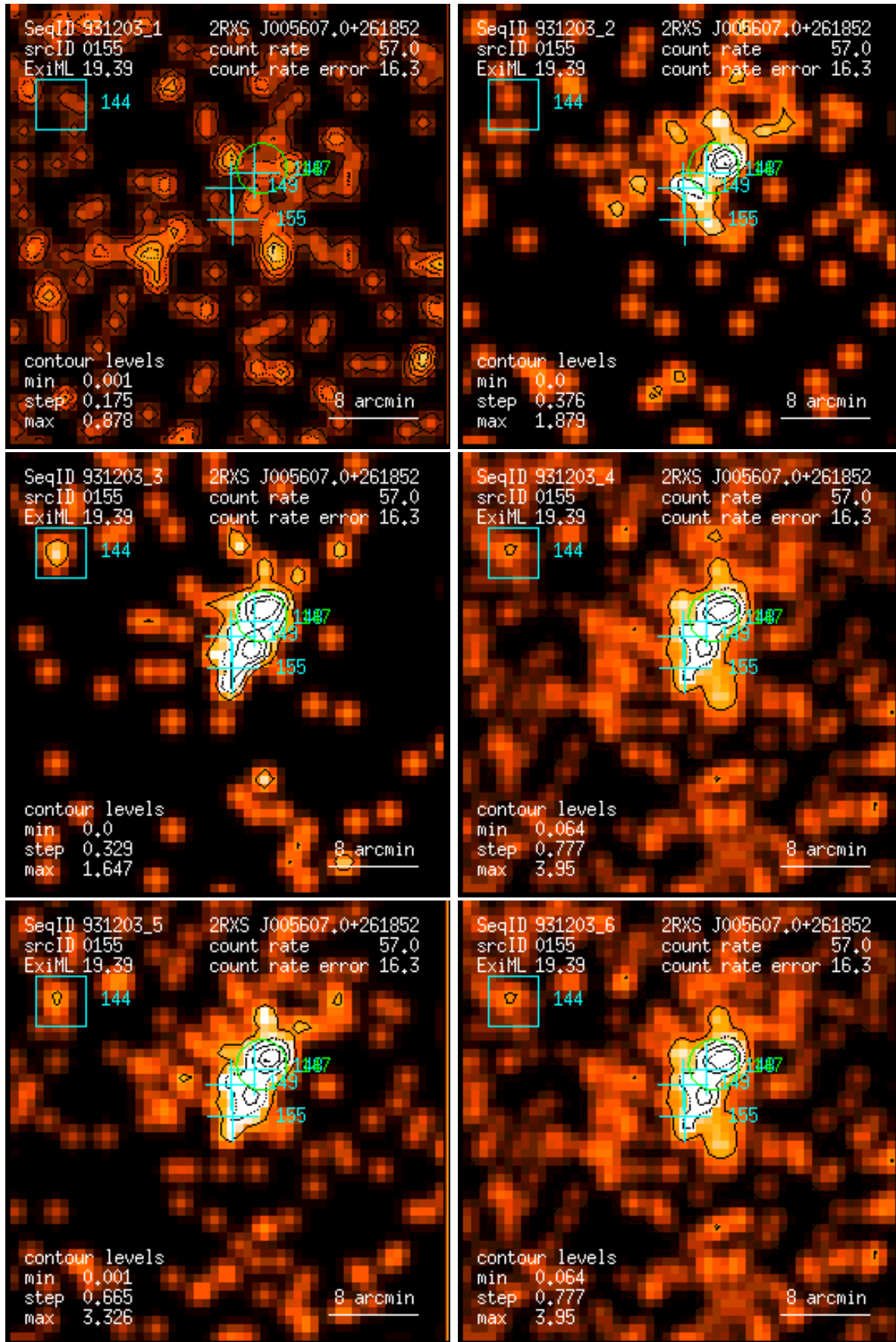
Figure 155: RASS 931203: detection 0155: band rate images, Gaussian filter: (1) PSPC channels 11 – 41, (2) 52 – 90, (3) 91 – 201, (4) 11 – 235, (5) 52 – 201, (6) 11 – 201. Broad band rates in counts/ks. Band rate contour levels in counts/ks/arcmin 2 .
