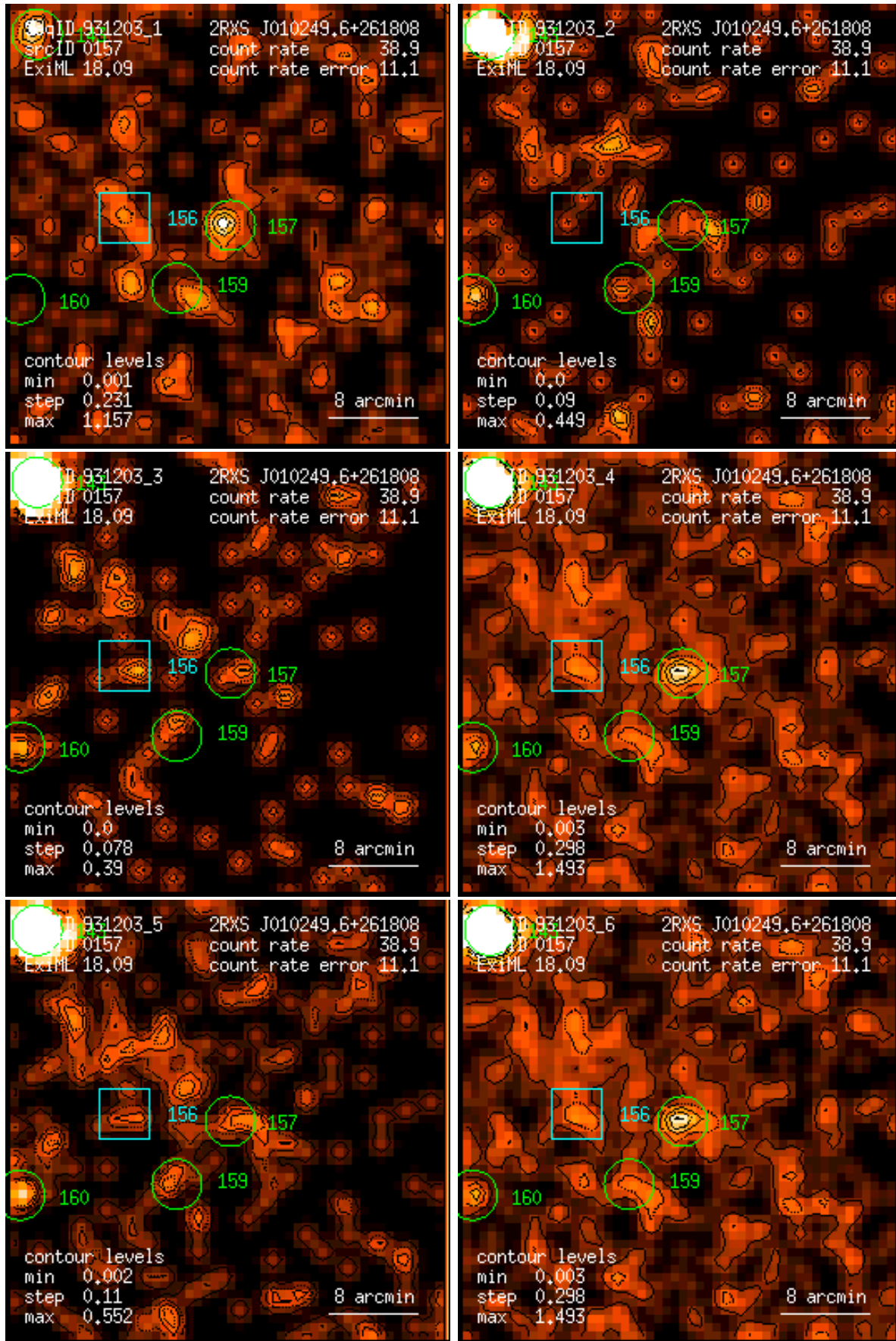
Figure 157: RASS 931203: detection 0157: band rate images, Gaussian filter: (1) PSPC channels 11 – 41, (2) 52 – 90, (3) 91 – 201, (4) 11 – 235, (5) 52 – 201, (6) 11 – 201. Broad band rates in counts/ks. Band rate contour levels in counts/ks/arcmin 2 .
